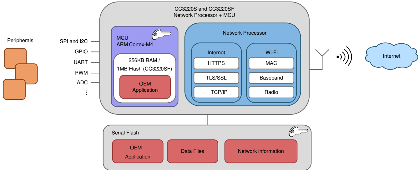
图 9-1. CC3220S and CC3220SF High-Level Structure
