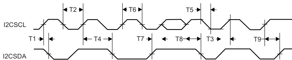
图 8-13. I 2 C Timing Diagram
