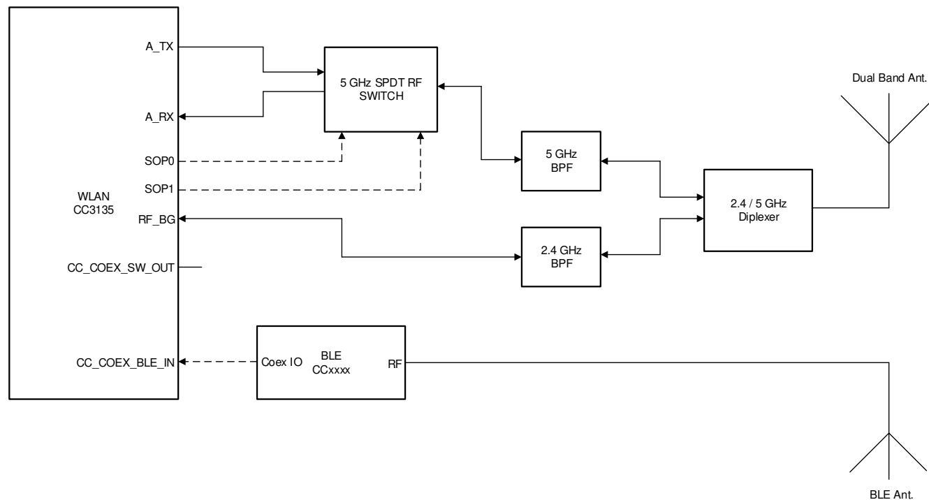
图 9-4. Dual Antenna Coexistence Solution with 5GHz Wi-Fi®
