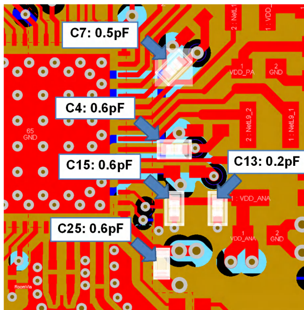
图 9-9. Ground Routing for Input Decoupling Capacitors
