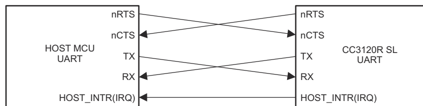
图 7-17. Typical 5-Wire UART Topology
