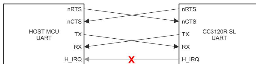
图 7-18. 4-Wire UART Configuration
