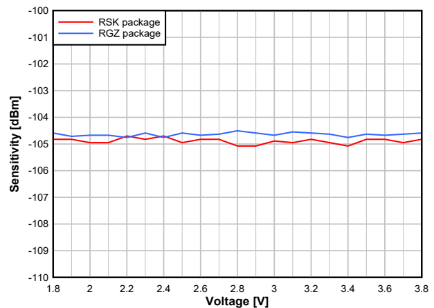
图 7-15. Sensitivity vs. Supply Voltage (VDD) (250kbps, 2.44GHz)
