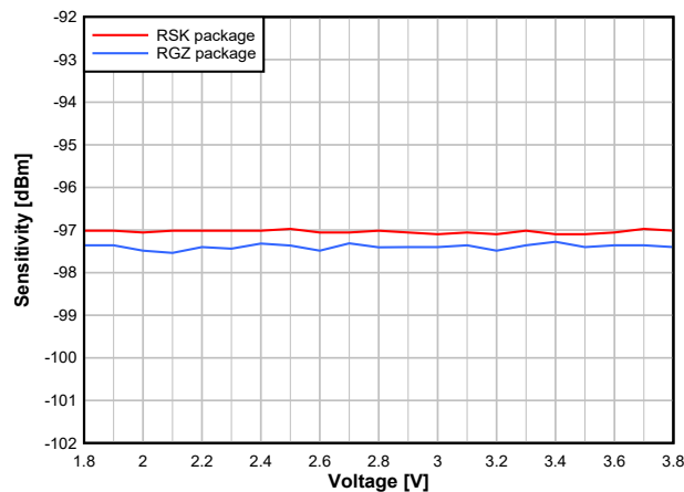
图 7-14. Sensitivity vs. Supply Voltage (VDD) (BLE 1Mbps, 2.44GHz)
