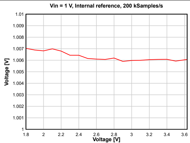
图 8-26. ADC Accuracy versus VDD
