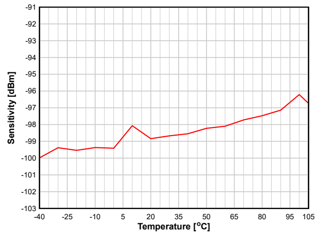
图 8-17. Sensitivity vs. Temperature (250 kbps, 2.44 GHz)
