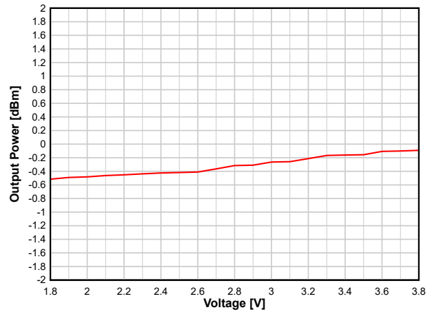
图 8-24. Output Power vs. Supply Voltage (VDD5) (BLE 1 Mbps, 2.44 GHz, 0 dBm)
