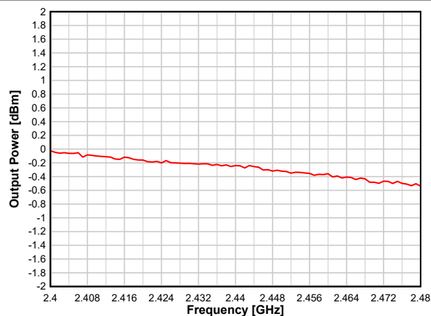
图 8-27. Output Power vs. Frequency (BLE 1 Mbps, 0 dBm)
