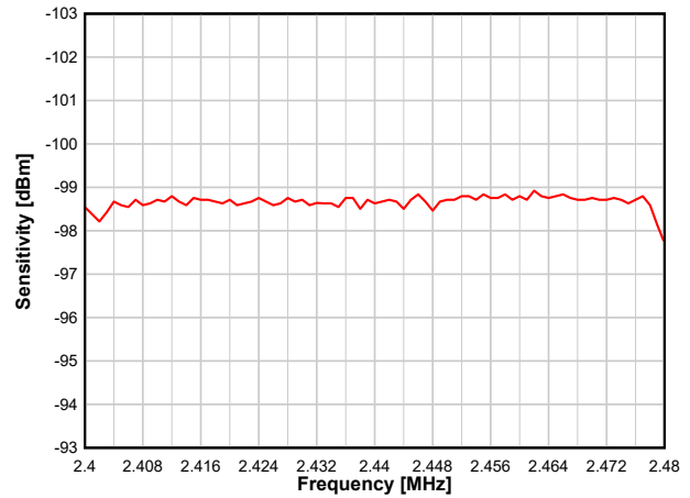
图 8-15. Sensitivity vs. Frequency (250 kbps)
