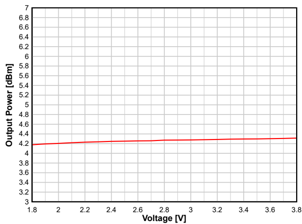
图 8-25. Output Power vs. Supply Voltage (VDD5) (BLE 1 Mbps, 2.44 GHz, +5 dBm)
