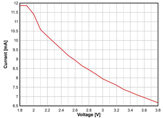
图 8-11. TX Current vs. Supply Voltage (VDD5) (BLE 1 Mbps, 2.44 GHz, 0 dBm)
