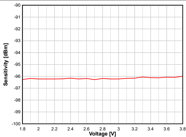
图 8-18. Sensitivity vs. Supply Voltage (VDD5) (BLE 1 Mbps, 2.44 GHz)
