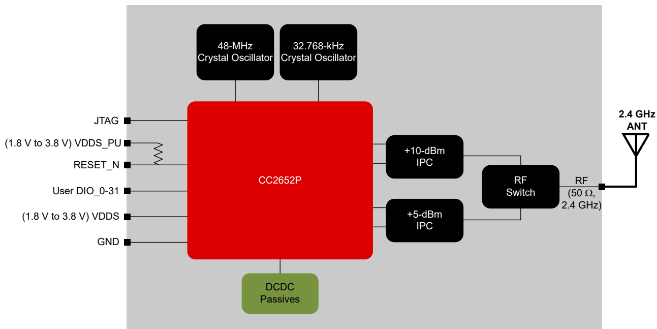
图 4-1. CC2652PSIP Block Diagram
