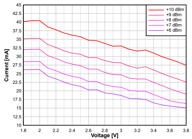
图 8-13. TX Current vs. Supply Voltage (VDD5) (BLE 1 Mbps, 2.44 GHz, +10 dBm PA)
