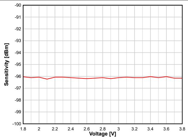
图 8-19. Sensitivity vs. Supply Voltage (VDD5) (BLE 1 Mbps, 2.44 GHz, DCDC Off)
