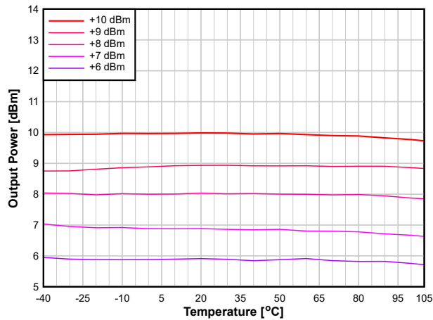
图 8-23. Output Power vs. Temperature (BLE 1 Mbps, 2.44 GHz, +10 dBm)
