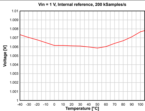
图 8-34. ADC Accuracy vs. Temperature
