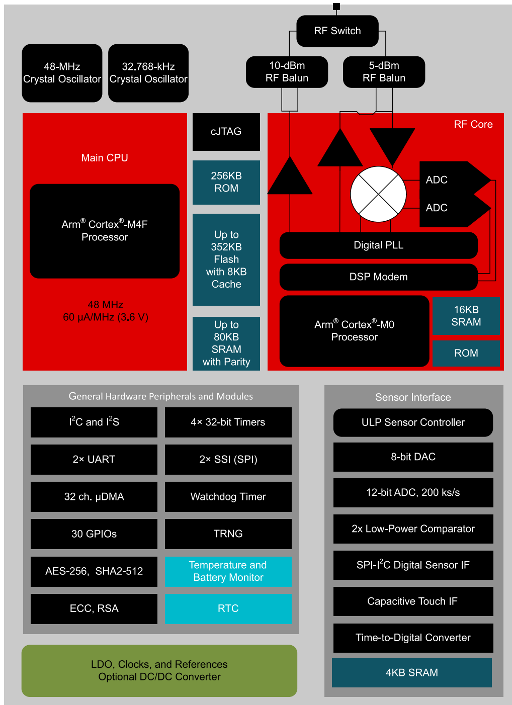
图 4-2. CC2652PSIP Hardware Overview
