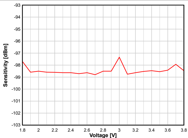
图 8-20. Sensitivity vs. Supply Voltage (VDD) (250 kbps, 2.44 GHz)
