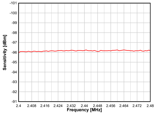
图 8-14. Sensitivity vs. Frequency (BLE 1 Mbps)
