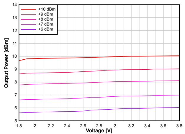
图 8-26. Output Power vs. Supply Voltage (VDD5) (2.44 GHz, +10 dBm PA)
