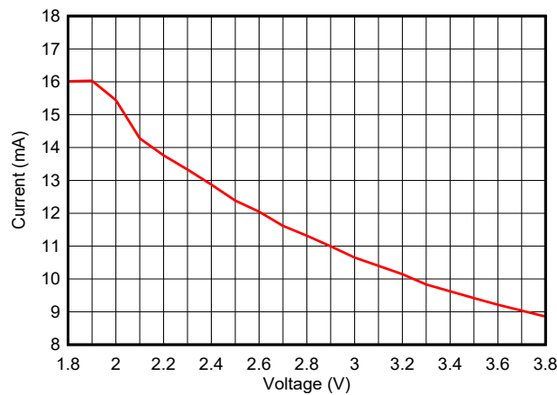
图 8-12. TX Current vs. Supply Voltage (VDD5) (BLE 1 Mbps, 2.44 GHz, +5 dBm)
