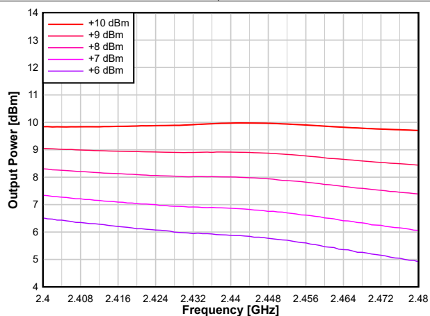
图 8-29. Output Power vs. Frequency (BLE 1Mbps, +10 dBm PA)
