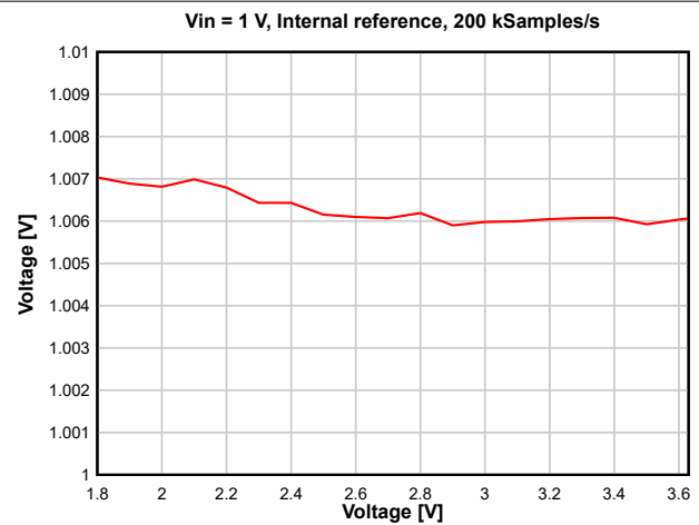
图 8-35. ADC Accuracy vs. Supply Voltage (VDD5)
