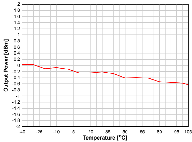
图 8-21. Output Power vs. Temperature (BLE 1 Mbps, 2.44 GHz, 0 dBm)
