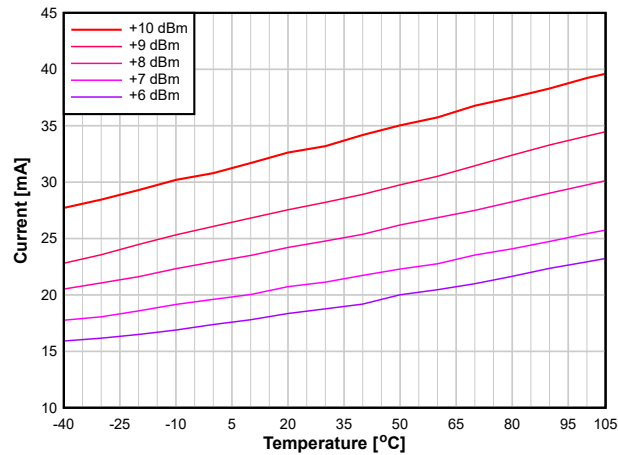
图 8-10. TX Current vs. Temperature (BLE 1 Mbps, 2.44 GHz, +10 dBm)
