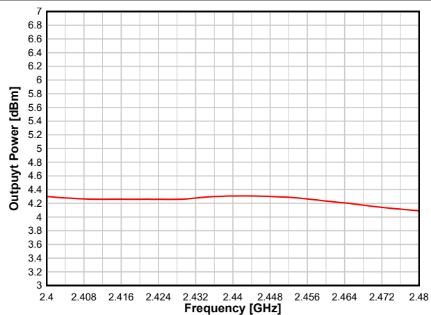
图 8-28. Output Power vs. Frequency (BLE 1 Mbps, +5 dBm)
