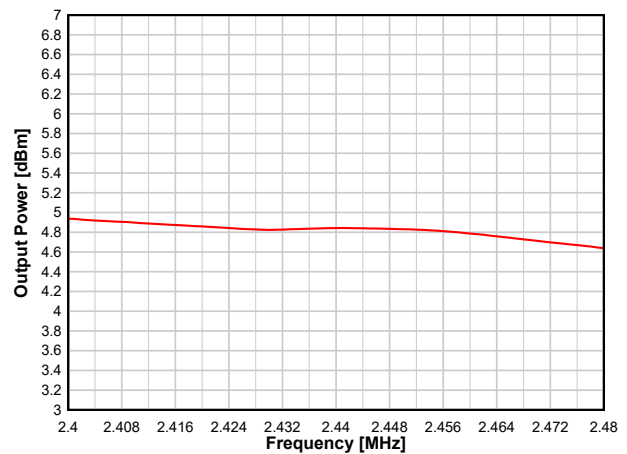
图 8-24. Output Power vs. Frequency (BLE 1 Mbps, 2.44 GHz, +5 dBm)
