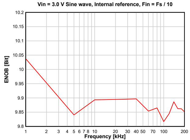
图 8-26. ENOB vs. Sampling Frequency
