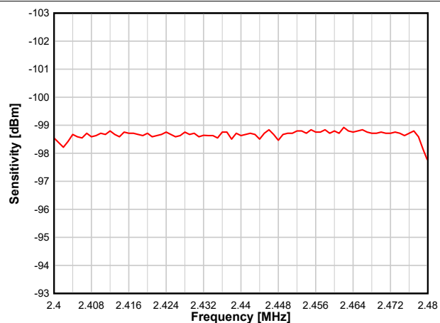
图 8-13. Sensitivity vs. Frequency (250 kbps, 2.44 GHz)
