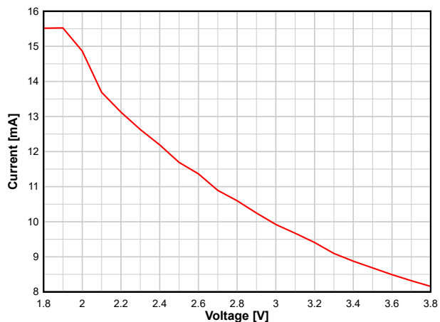
图 8-11. TX Current vs. Supply Voltage (VDDS) (BLE 1 Mbps, 2.44 GHz, +5 dBm)
