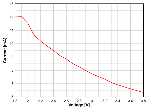
图 8-10. TX Current vs. Supply Voltage (VDDS) (BLE 1 Mbps, 2.44 GHz, 0 dBm)
