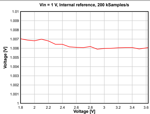
图 8-30. ADC Accuracy vs. Supply Voltage (VDDS)
