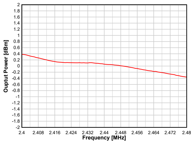
图 8-23. Output Power vs. Frequency (BLE 1 Mbps, 2.44 GHz, 0 dBm)
