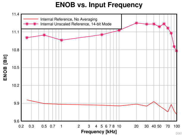
图 8-33. ENOB vs. Input Frequency
