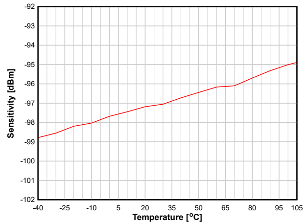
图 8-12. Sensitivity vs. Temperature (BLE 1 Mbps, 2.44 GHz)
