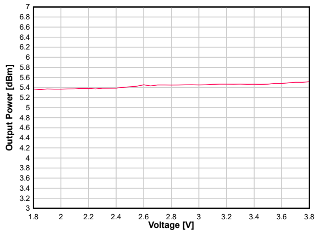
图 8-19. Output Power vs. Supply Voltage (VDD5) (BLE 1 Mbps, 2.44 GHz, +5dBm)
