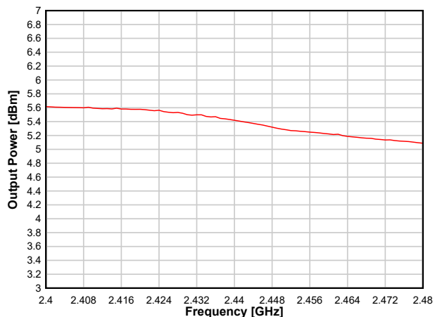
图 8-21. Output Power vs. Frequency (BLE 1 Mbps, +5dBm)
