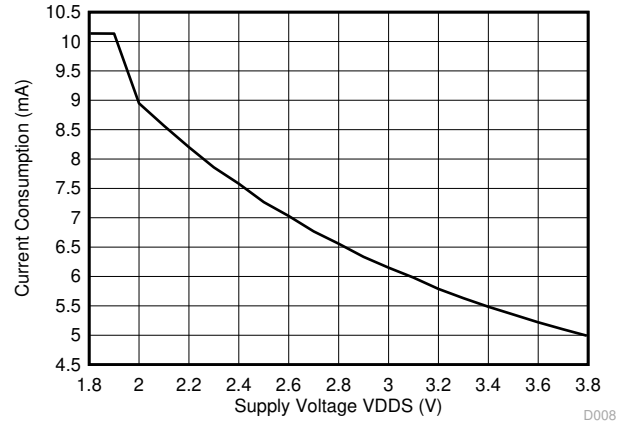
图 7-11. RX Mode Current vs Supply Voltage (VDD5)
