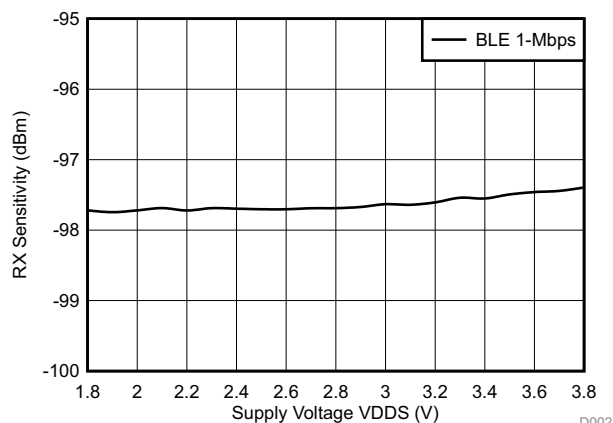
图 7-5. Bluetooth Low Energy Sensitivity vs Supply Voltage (VDD5)
