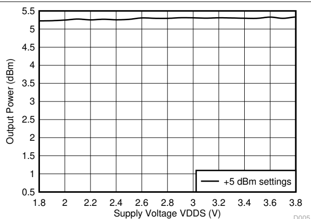
图 7-8. TX Output Power vs Supply Voltage (VDD5)
