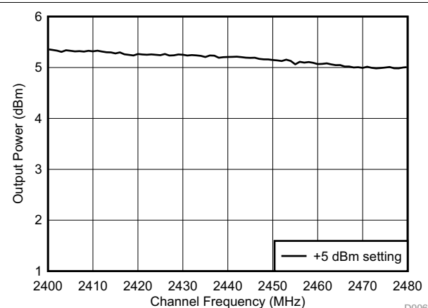
图 7-9. TX Output Power vs Channel Frequency
