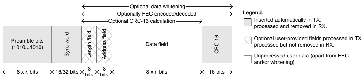
Figure 11: Packet Format
