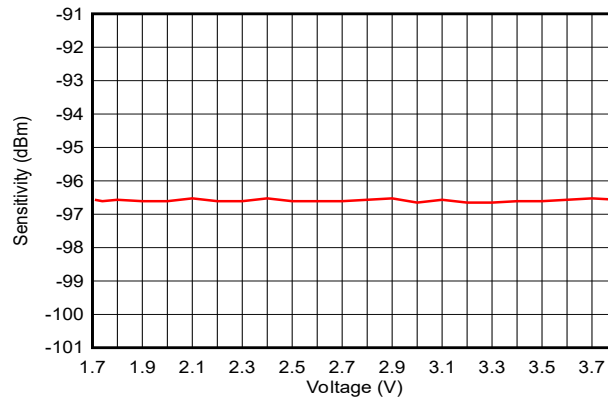
图 7-20. Sensitivity vs. Supply Voltage (VDD5) (BLE 1Mbps, 2.44GHz, DCDC Off)
