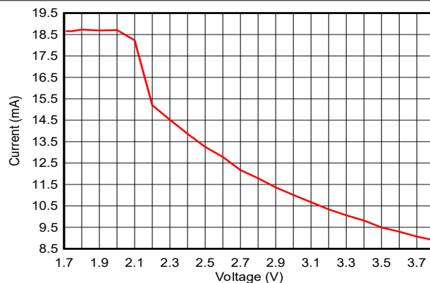
图 7-13. TX Current vs. Supply Voltage, VDD (BLE 1Mbps, 2.44GHz, +8dBm)
