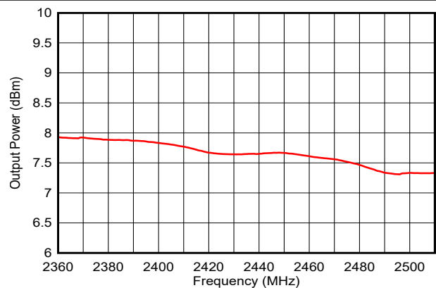
图 7-26. Output Power vs. Frequency (BLE 1Mbps, +8dBm)
