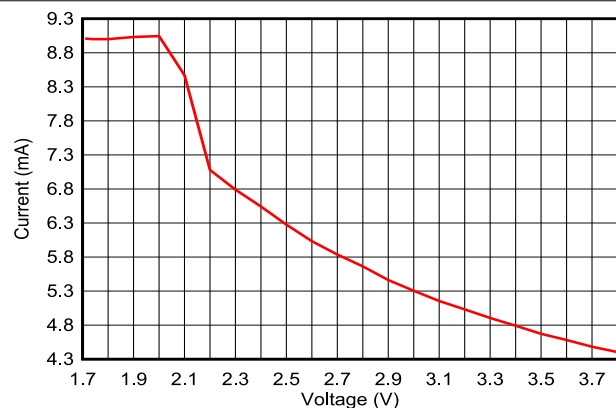
图 7-12. TX Current vs. Supply Voltage, VDD (BLE 1Mbps, 2.44GHz, 0dBm)
