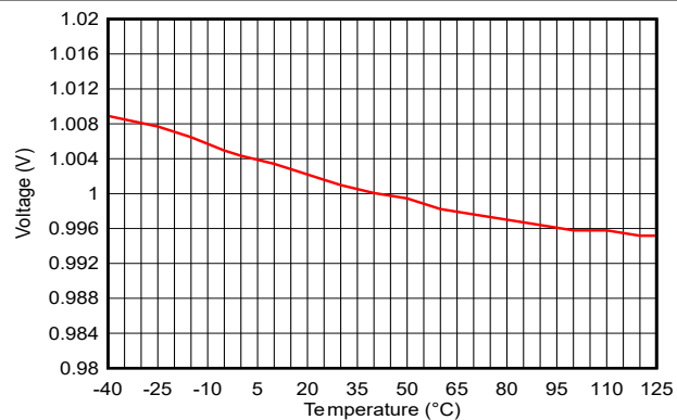
图 7-33. ADC Accuracy vs. Temperature ( V_{in}=1V , Internal Reference, 200ksps)
