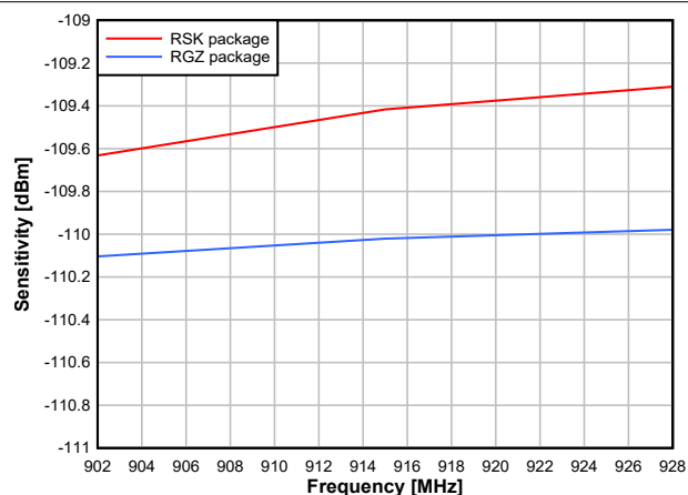
图 7-15. Sensitivity vs. Frequency (50kbps, 915MHz)
