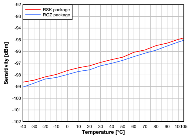
图 7-19. Sensitivity vs. Temperature (BLE 1 Mbps, 2.44GHz)
