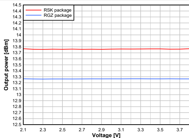
图 7-28. Output Power vs. Supply Voltage (VDD5) (50kbps, 868.3MHz, +14dBm)
