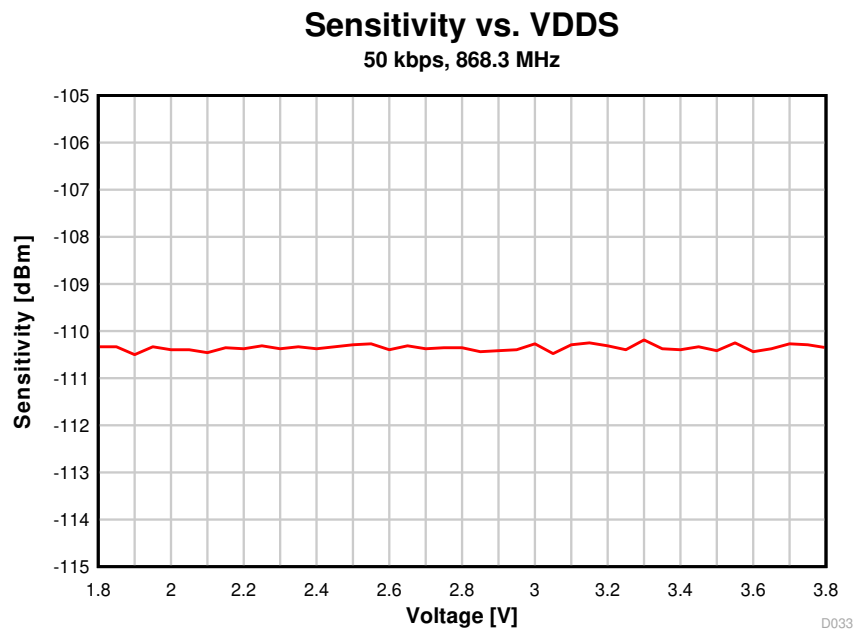
图 8-24. Sensitivity vs. Supply Voltage (VDD) (50 kbps, 868.3 MHz)
