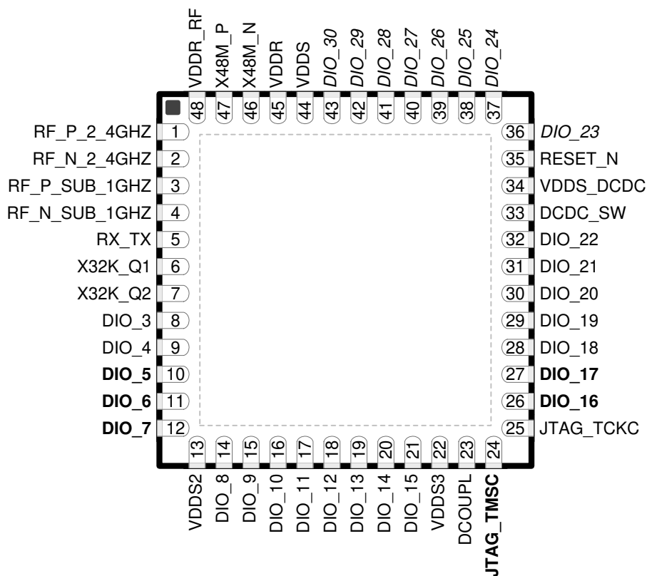
图 7-1. RGZ (7-mm x 7-mm) Pinout, 0.5-mm Pitch (Top View)
