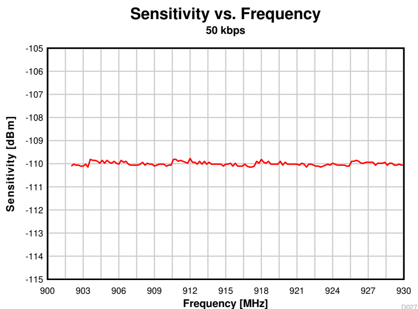
图 8-18. Sensitivity vs. Frequency (50 kbps, 915 MHz)
