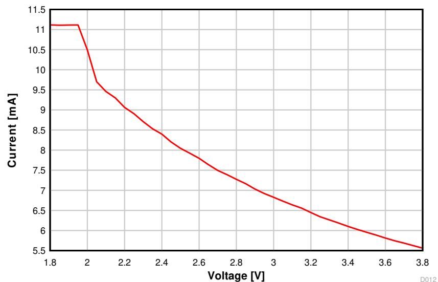
图 8-10. RX Current vs. Supply Voltage (VDD5) (50 kbps, 868.3 MHz)
