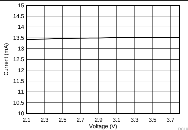
Figure 5-29. TX Maximum Output Power vs VDD5, 868 MHz
