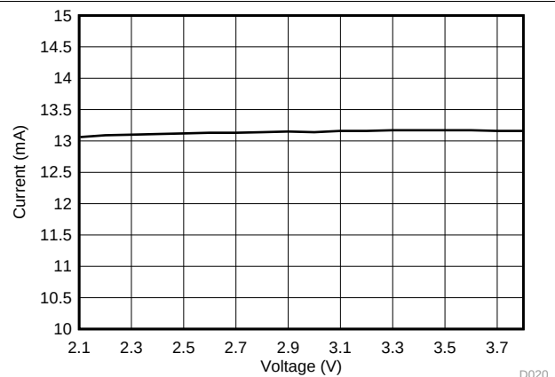
Figure 5-30. TX Maximum Output Power vs VDD5, 915 MHz
