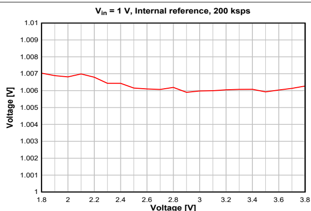
图 7-24. ADC Accuracy vs. Supply Voltage (VDD5)
