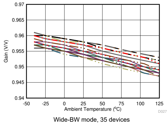
图 6-52. Buffer Gain vs Temperature
