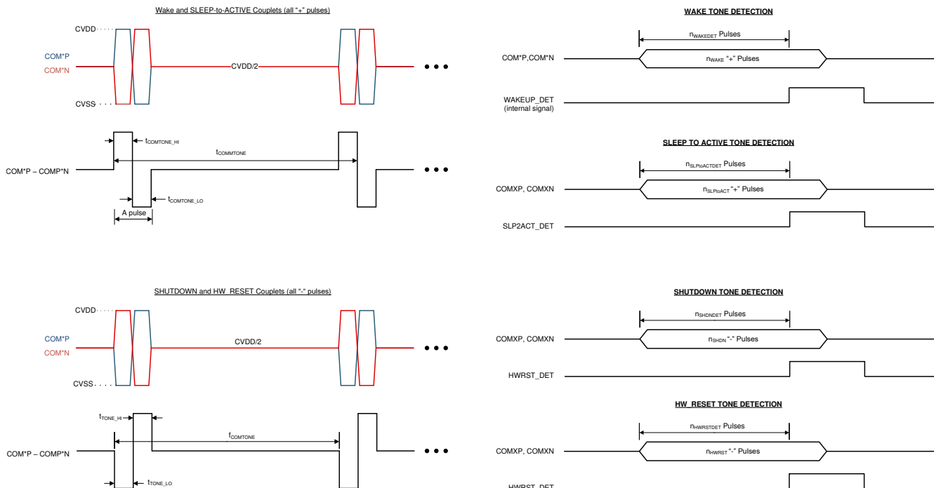
图 8-48. Communication Tones
