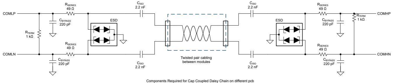
图 9-13. Capacitor Isolation on Different PCB
