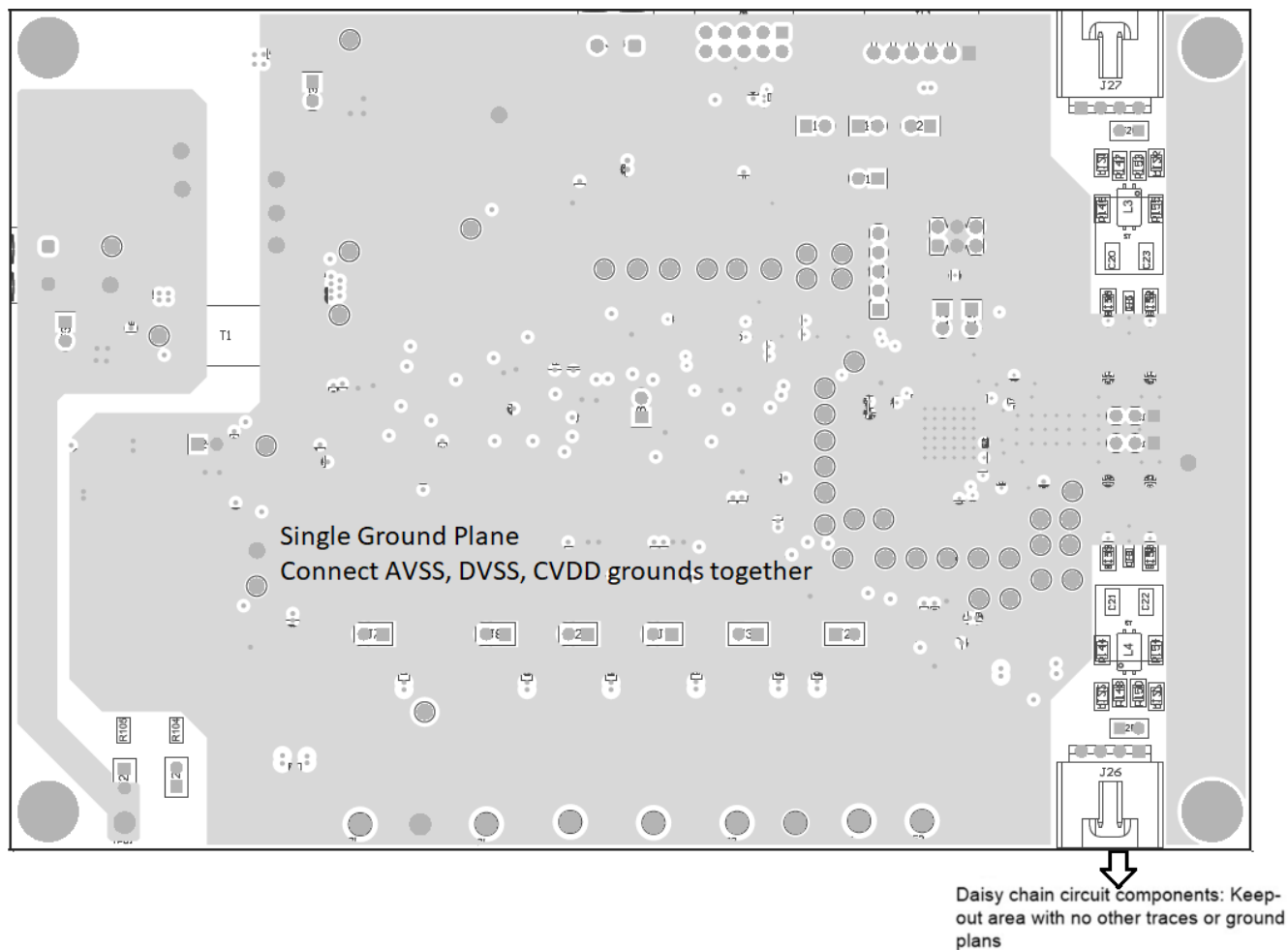
图 11-5. Thlr3 Layer with Single Ground Plane
