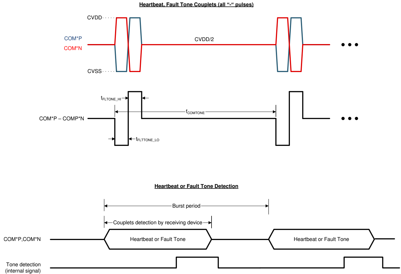
图 8-38. Heartbeat and Fault Tone
