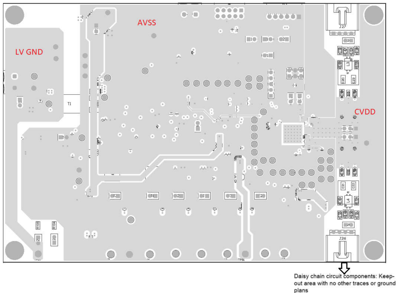
图 11-4. Second Layer with Solid, Separate Ground Planes
