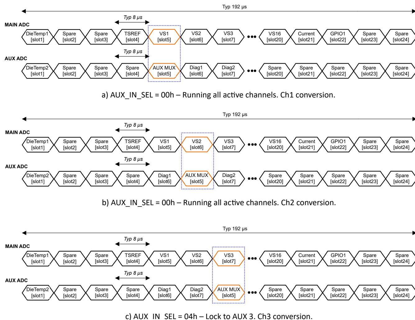
图 8-9. Synchronization Between MAIN and AUX ADC Sampling
