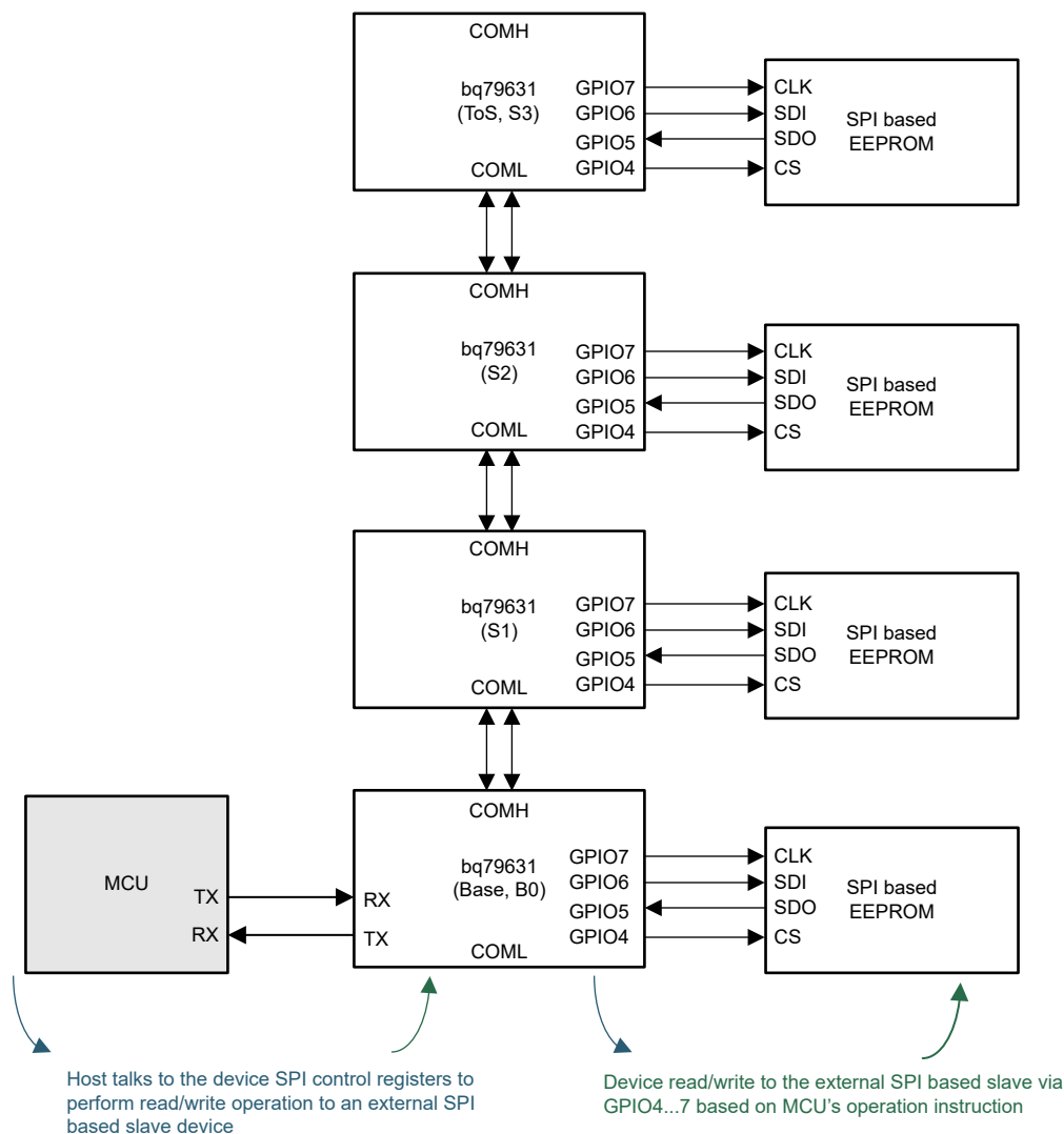
图 8-32. SPI Master Stack Configuration
