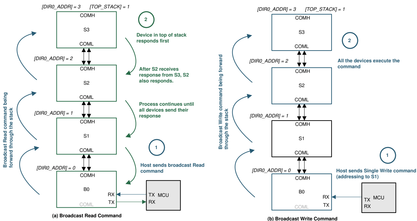
图 8-23. Broadcast Read/Write
