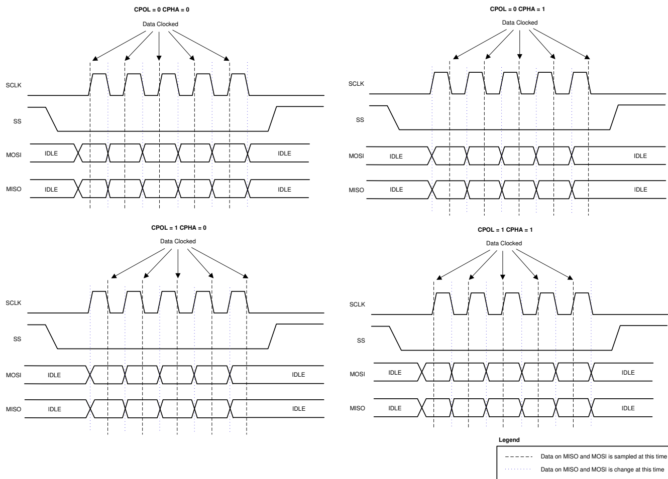
图 8-33. SPI Master CPOL and CPHA
