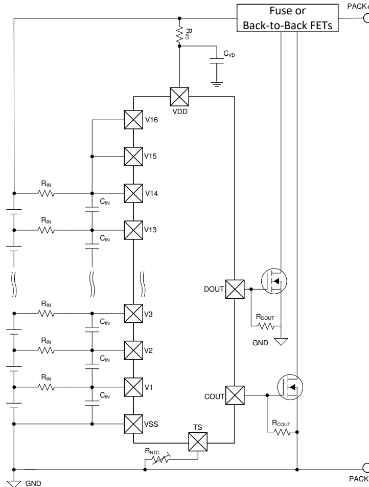
图 8-3. 14-Series Cell Configuration with Active High 6V Option
