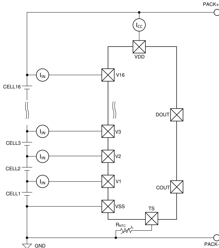
图 8-2. Configuration for IC Current Consumption Test
