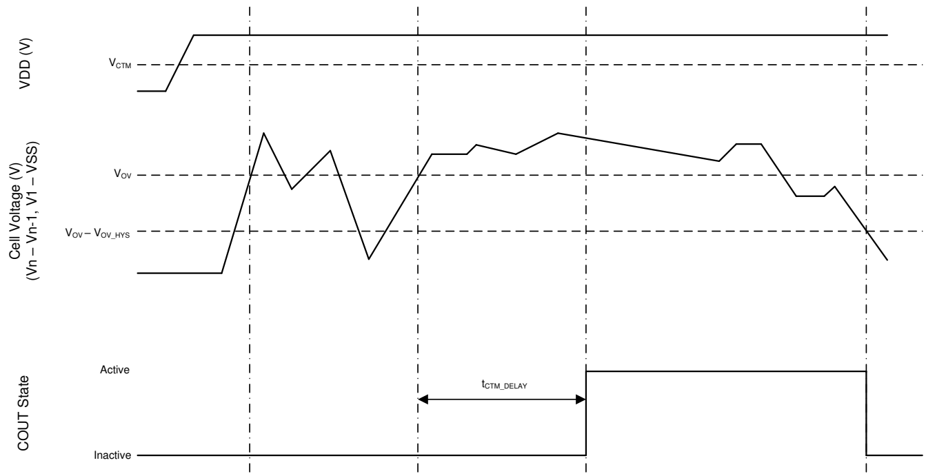
图 7-3. Timing for Customer Test Mode
