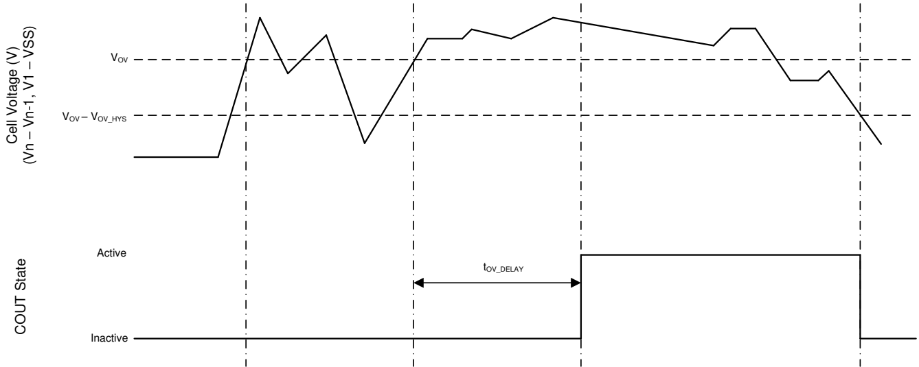
图 7-1. Timing for Overvoltage Sensing
