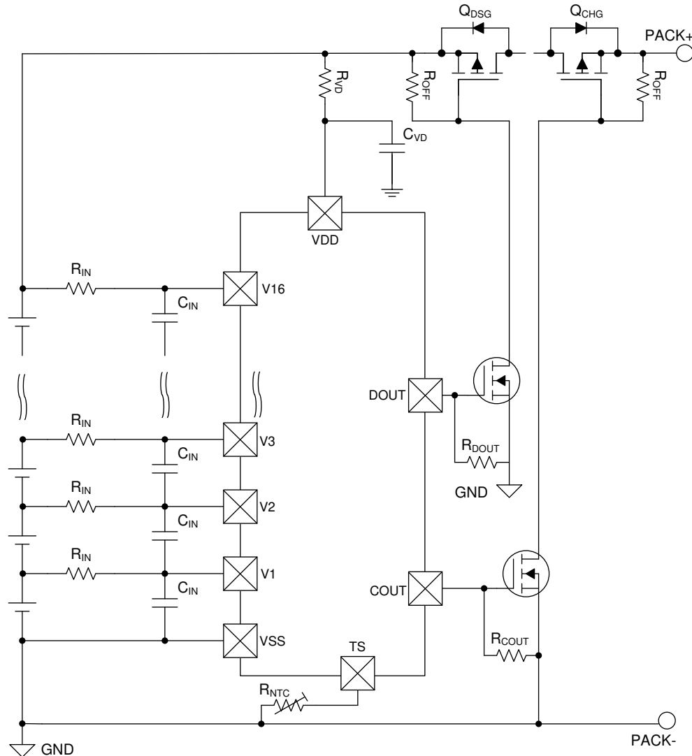
图 8-1. Application Configuration
