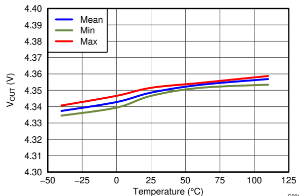
图 7-1. Overvoltage Threshold (OVT) vs. Temperature
