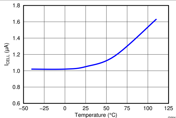
图 7-4. I_{CELL} vs. Temperature at V_{CELL} = 9.2\text{ V}
