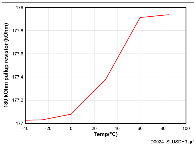
图 7-22. Thermistor Pullup Resistance vs. Temperature (180-k \Omega Setting)
