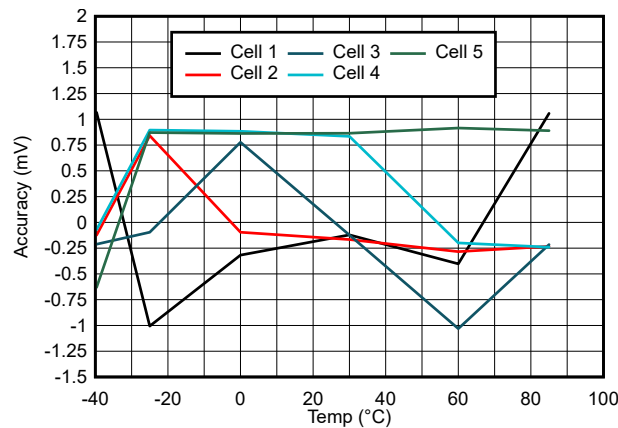
图 6-5. Cell Voltage Measurement Error vs Temperature with Cell Voltage = 2.5 V
