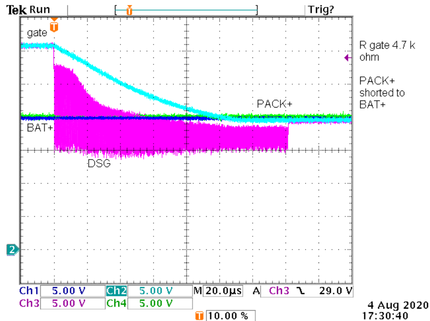
图 8-10. A Slower Turn-Off Case Using a 4.7-k \Omega Series Gate Resistor, and the PACK+ Connector Shorted to the Top of the Stack
