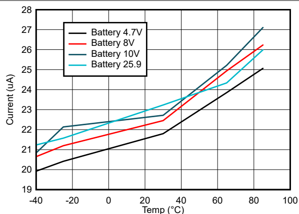
图 6-27. BAT Current in SLEEP2 (SRC Follower) Mode vs Temperature
