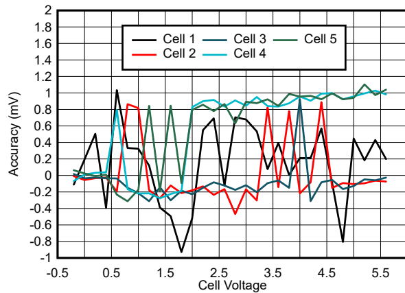
图 6-3. Cell Voltage Measurement Error at 25°C Across Input Range
