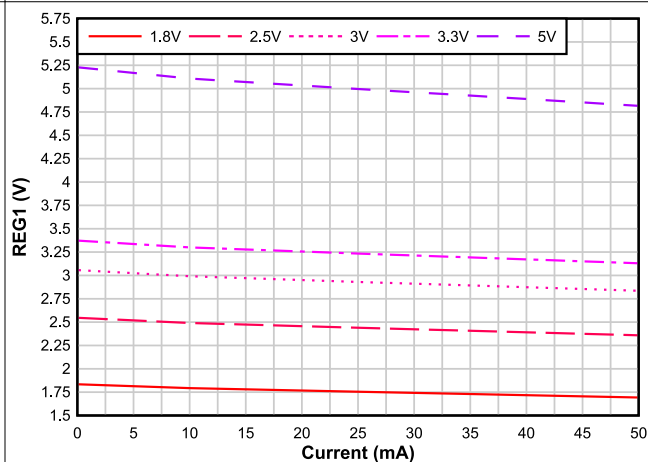
图 6-18. REG1 Voltage vs Load at 25°C
