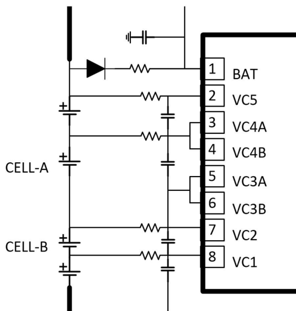
图 7-2. Terminating an Unused Cell Input Pin
