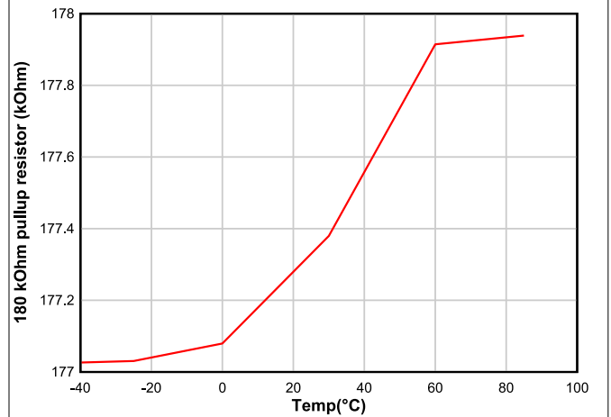
图 6-20. Thermistor Pullup Resistance vs Temperature (180-kΩ Setting)
