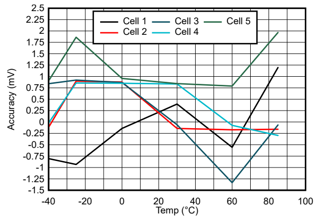
图 6-6. Cell Voltage Measurement Error vs Temperature with Cell Voltage = 3.5 V
