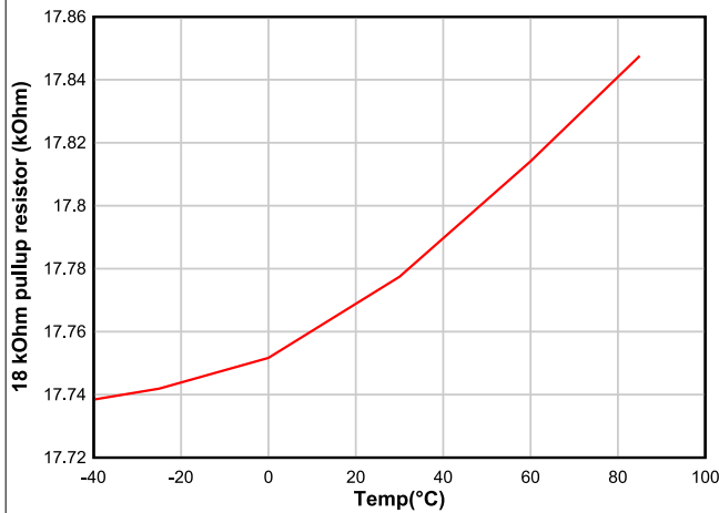
图 6-19. Thermistor Pullup Resistance vs Temperature (18-kΩ Setting)
