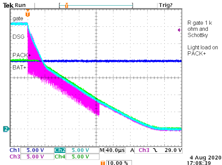
图 8-8. Moderate Speed DSG FET Turn-Off, Using a 1-k \Omega Series Gate Resistor, and a Light Load on PACK+.
