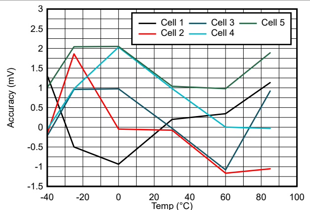
图 6-8. Cell Voltage Measurement Error vs Temperature with Cell Voltage = 5.5 V
