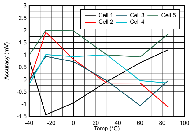
图 6-7. Cell Voltage Measurement Error vs Temperature with Cell Voltage = 4.5 V
