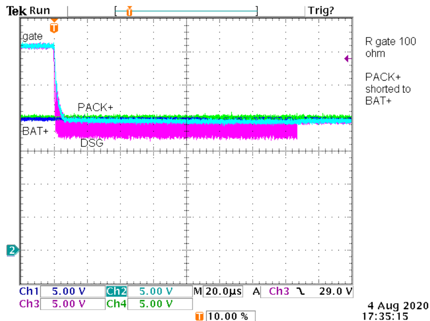
图 8-11. A Fast Turn-Off Case with a 100- \Omega Series Gate Resistor
