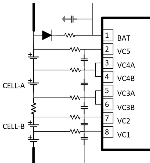
图 7-1. Using Cell Input Pins for Interconnect Measurement
