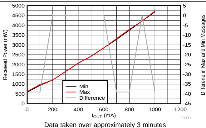
Figure 22. 0-mA to 1000-mA Step on a WPC TX
