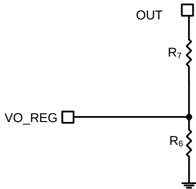
Figure 8. VO_REG Network
