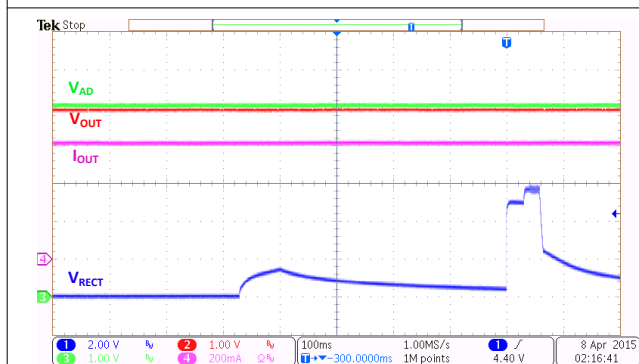
Figure 10-9. Wireless Power Start-Up With V_{AD} = 5\text{ V} (EN1 = EN2 = LOW)
