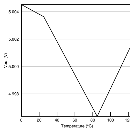
图 8-8. V OUT vs Temperature
