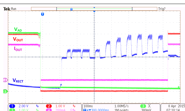
Figure 10-8. Transition Between Wired Power and Wireless Power (EN1 = EN2 = LOW)
