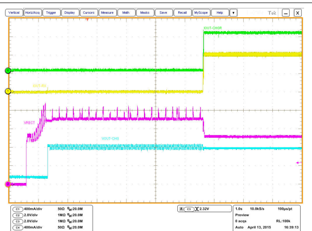
图 10-13. System Start-Up With Battery Inserted After Wireless Power is Enabled (1 s / division)
