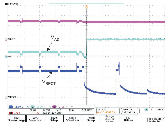
图 8-16. On-the-Go Enabled ( V_{OTG} = 3.5\text{ V} ) (3)
