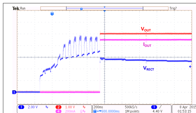
图 10-4. Start-Up With 900-mA Load
