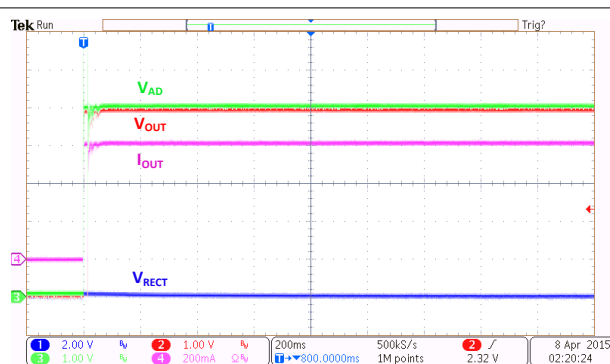
Figure 10-10. AD Power Start-Up With No Transmitter (EN1 = EN2 = LOW)
