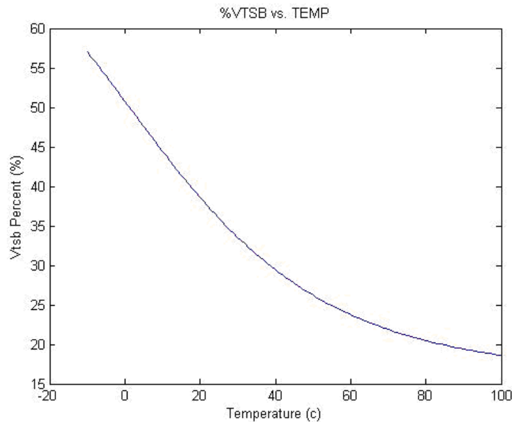
图 9-13. Example Solution for an NTC Resistor with R_O = 10 k \Omega and \beta = 3380
