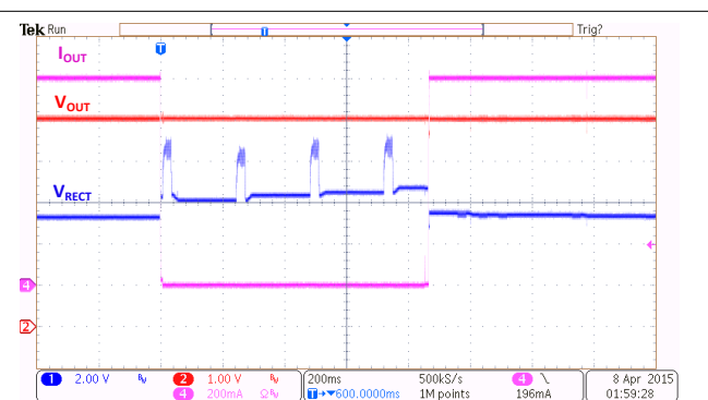
图 10-5. Load Transitions (1 A to 0 A to 1 A)
