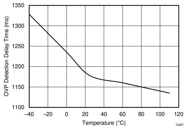
图 6-7. OVP Detection Delay Time Versus Temperature
