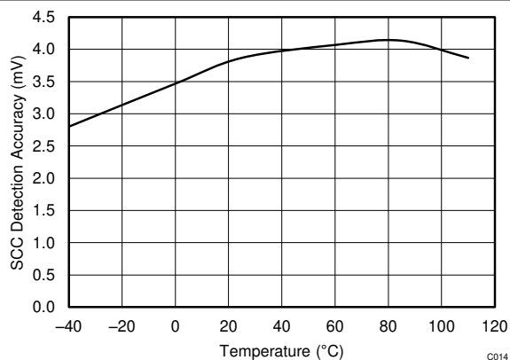
图 6-14. SCC Detection Accuracy Versus Temperature
