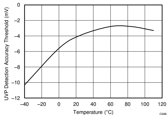
图 6-8. UVP Detection Accuracy Versus Temperature
