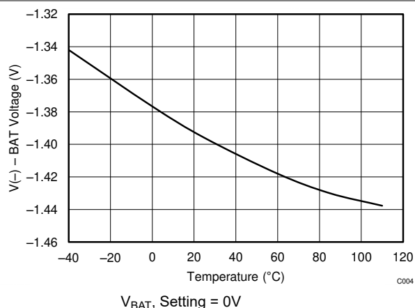
图 6-4. 0V Charging Allowed Versus Temperature
