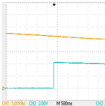
图 9-5. Initial Power Up, COUT
