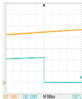
图 9-4. Initial Power Up, DOUT
