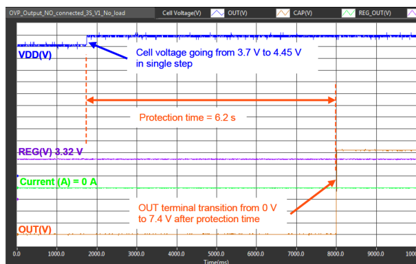
Figure 8-4. Overvoltage Protection
