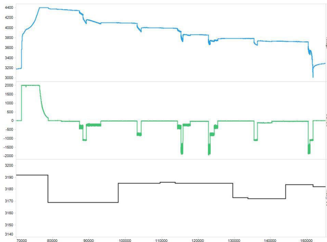
图 9-3. Full Charge Capacity Tracking (X-Axis Is Seconds)
