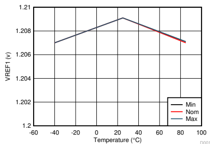
图 7-3. REF1 Voltage Versus Battery and Temperature
