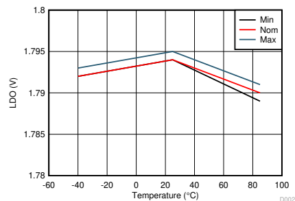
图 7-4. LDO Voltage Versus Battery and Temperature
