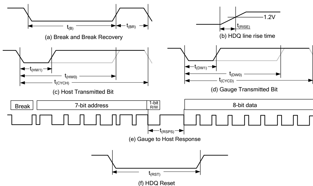
Figure 2. Timing Diagrams
