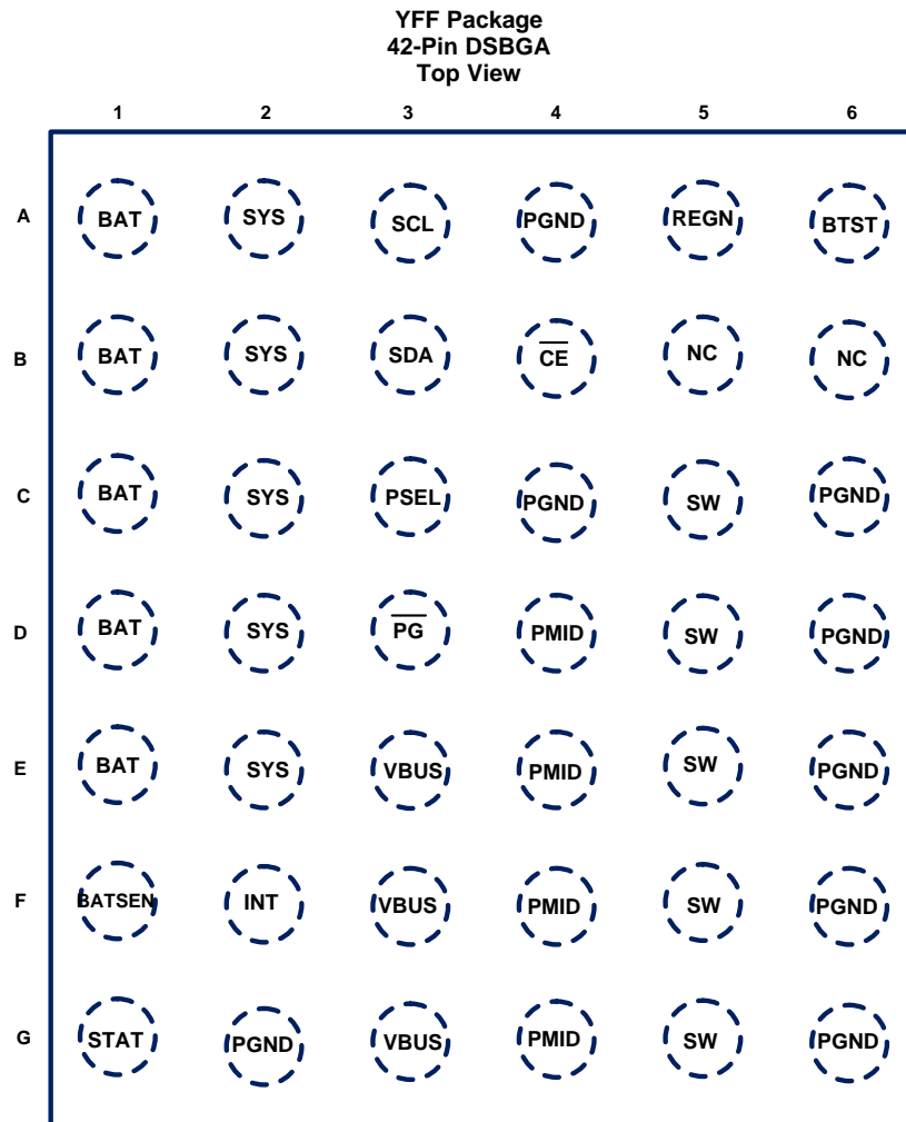
Pin Functions
