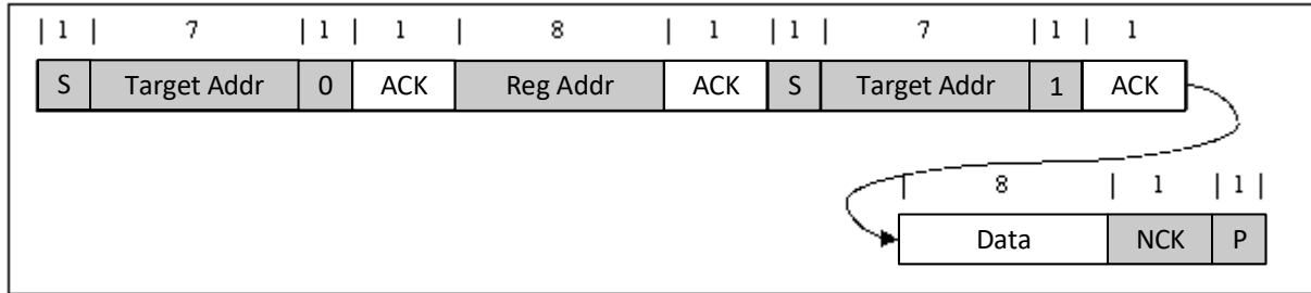
图 8-14. Single Read
