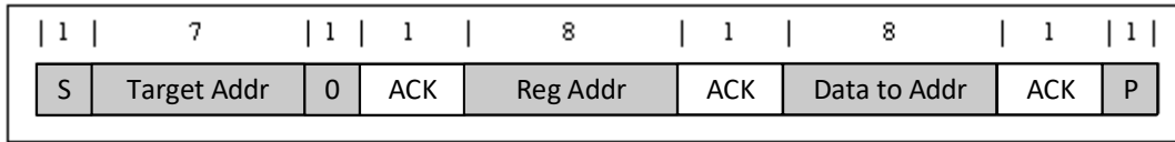
图 8-13. Single Write
