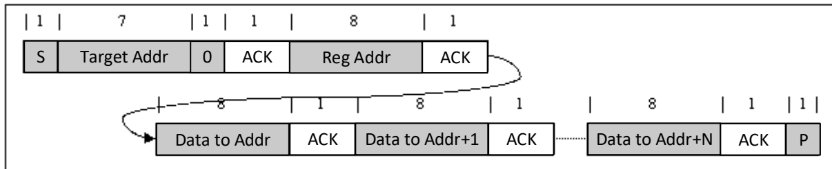
图 8-15. Multi-Write
