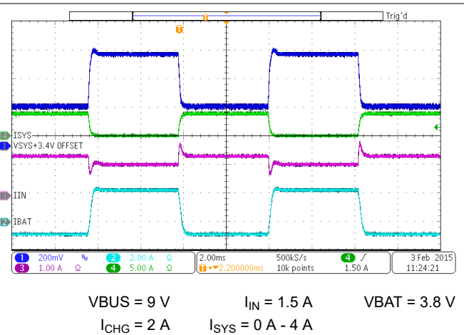
图 9-9. Load Transient During Supplement Mode
