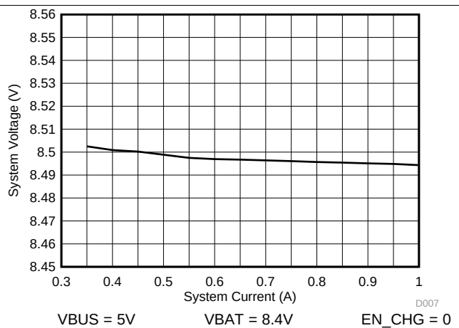
图 10. System Load Regulation After Charge Done
