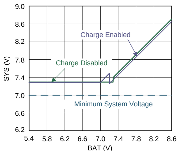
图 14. System Voltage vs. Battery Voltage
