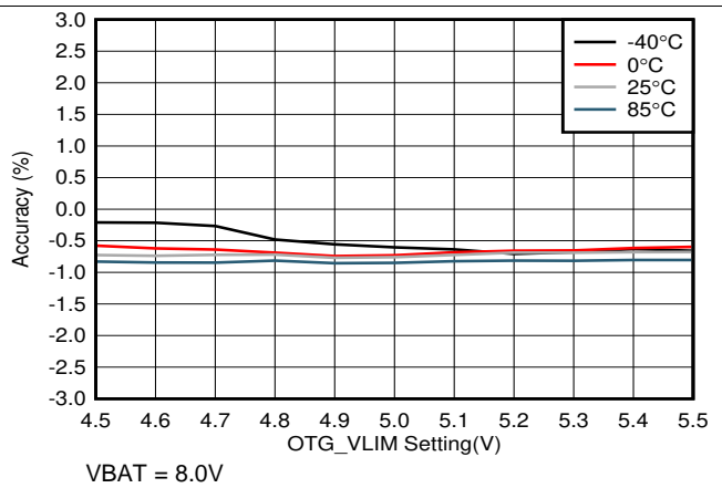
图 10. OTG VBUS Regulation vs. OTG_VLIM Setting
