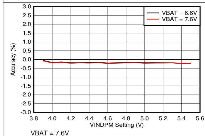
图 15. Input Voltage Limit Accuracy vs. VINDPM Setting
