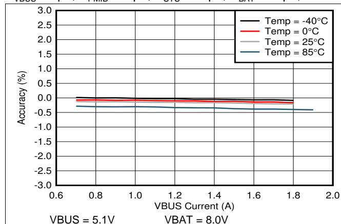
图 13. OTG Voltage Regulation vs. OTG BUS Current
