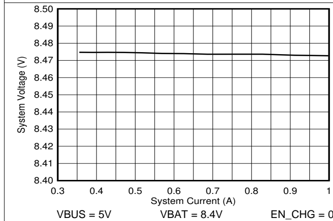
图 9. System Load Regulation After Charge Done
