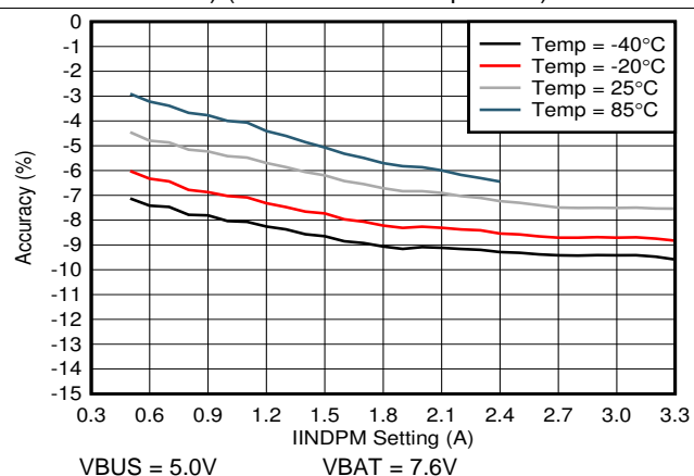
图 14. Input Current Limit Accuracy vs. IINDPM Setting
