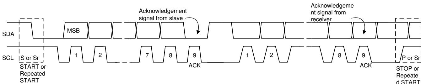
图 29. Data Transfer on the I 2 C Bus
