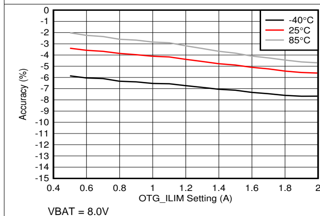
图 11. OTG IBUS Limit vs. OTG_ILIM Setting
