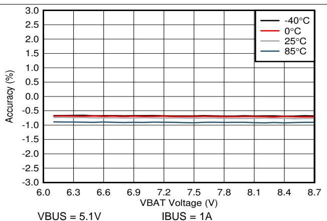
图 12. OTG Voltage Regulation vs. VBAT Voltage
