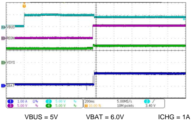
图 77. Adapter Power Up With Charge Enabled
