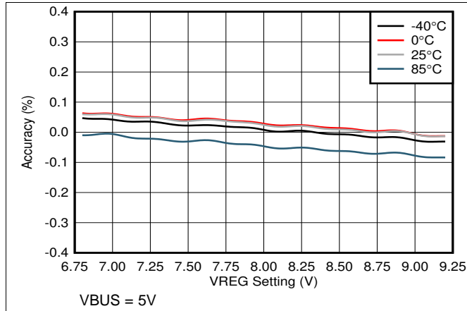
图 7. Battery Voltage Accuracy vs. VREG Setting
