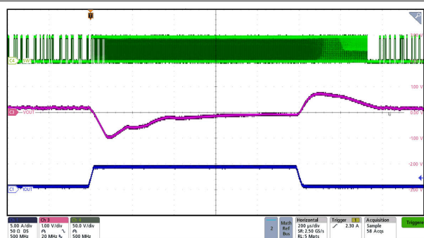
VAC = 48V VOUT = 36V ILOAD = 0.5A → 4.5A
