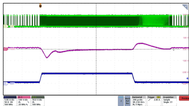
VAC = 48V VOUT = 28V ILOAD = 0.5A → 4.5A
