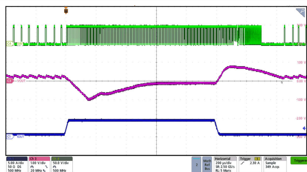
VAC = 48V VOUT = 48V ILOAD = 0.5A → 4.5A
