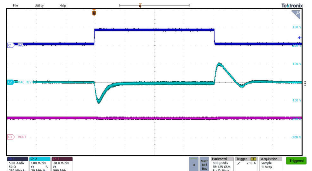
图 9-16. Reverse Mode Buck Transient Response
