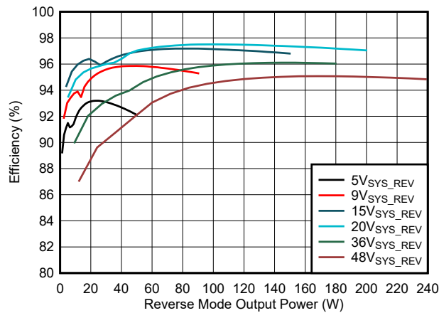
图 7-9. Reverse Mode Efficiency (5s battery configuration)
