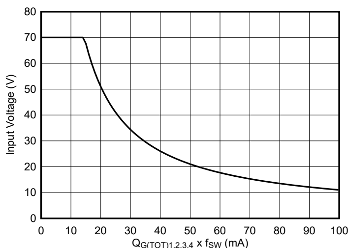
图 8-2. REGN LDO Safe Operating Area (SOA)
