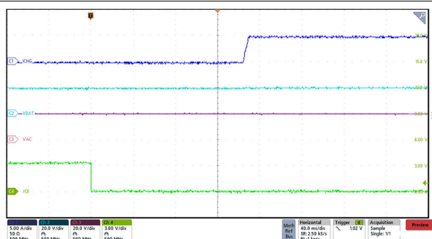
图 9-5. Charge Enable via I 2 C with 5-A ICHG
