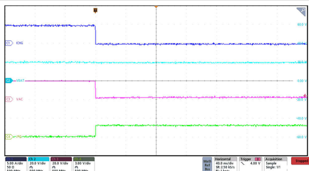
图 9-4. VAC Un-plug Power Down with 5-A ICHG
