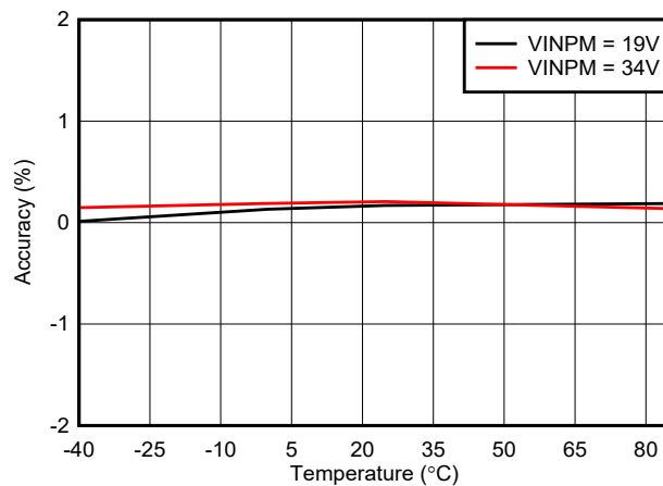
图 7-7. Input Voltage (VAC_DPM) Regulation Accuracy vs Temperature
