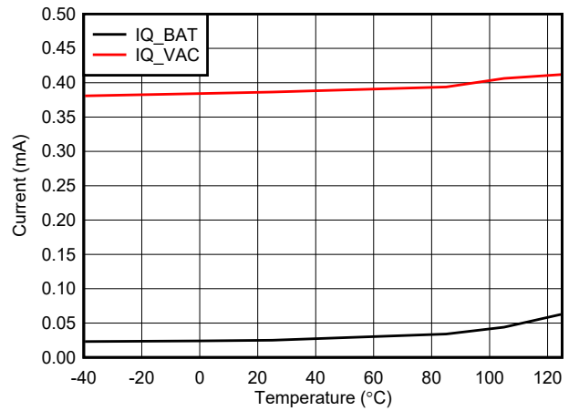
图 7-6. Battery and Input Quiescent Current vs Temperature with VBAT = 28 V
