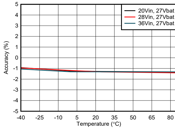
图 7-5. Charge Current Accuracy vs Temperature
