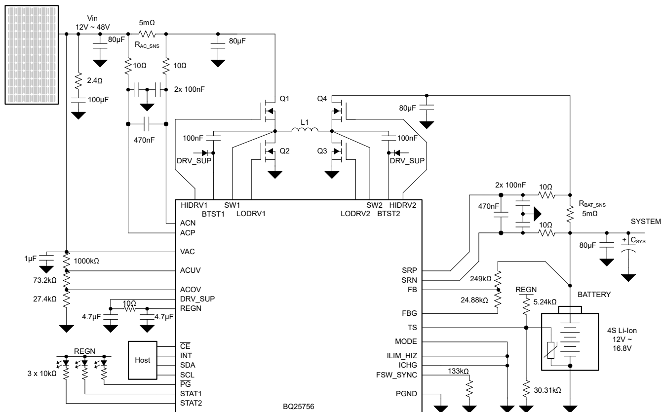
图 9-1. BQ25756: Solar Charging with Autonomous MPPT Algorithm to Charge 4s Battery with Maximum 15-A Charge Current
