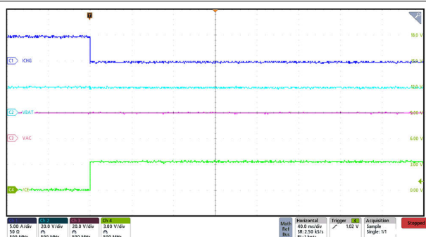
图 9-8. Charge Disable via \overline{CE} Pin with 5-A ICHG
