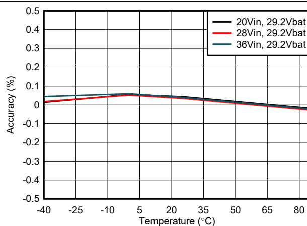
图 7-4. Charge Voltage Accuracy vs Temperature
