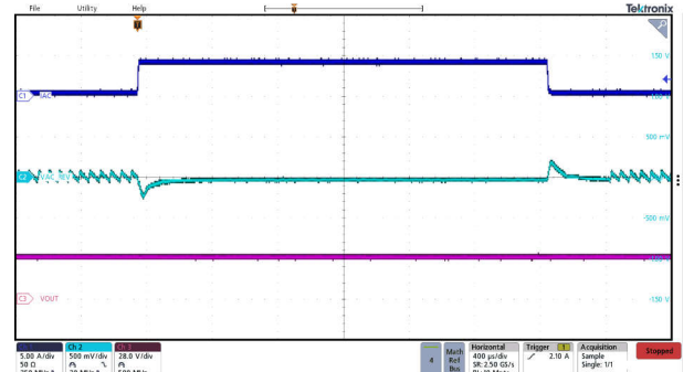
图 9-16. Reverse Mode Buck Transient Response
