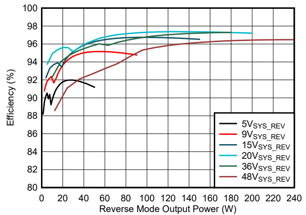
图 7-10. Reverse Mode Efficiency (7s battery configuration)
