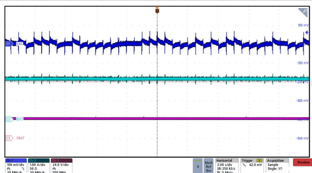
图 9-13. Max Power Point Tracking (MPPT) Perturb and Observe
