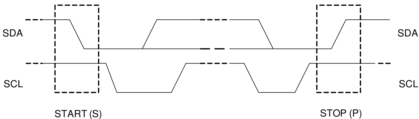
图 9-9. START and STOP Conditions
