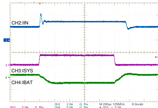
图 10-11. Switching During Buck Boost Mode
