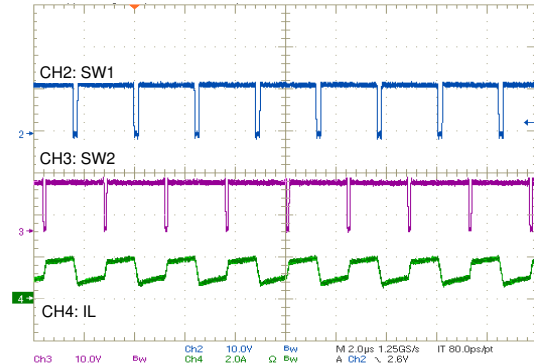
图 10-11. Switching During Buck Boost Mode
