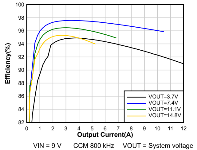
图 8-2. System Efficiency
