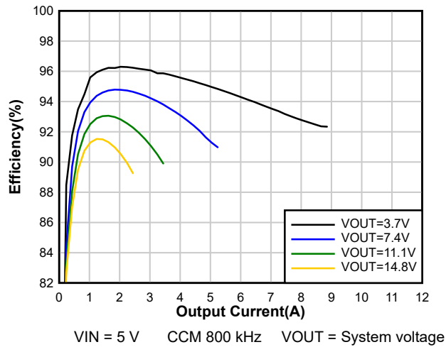
图 8-1. System Efficiency
