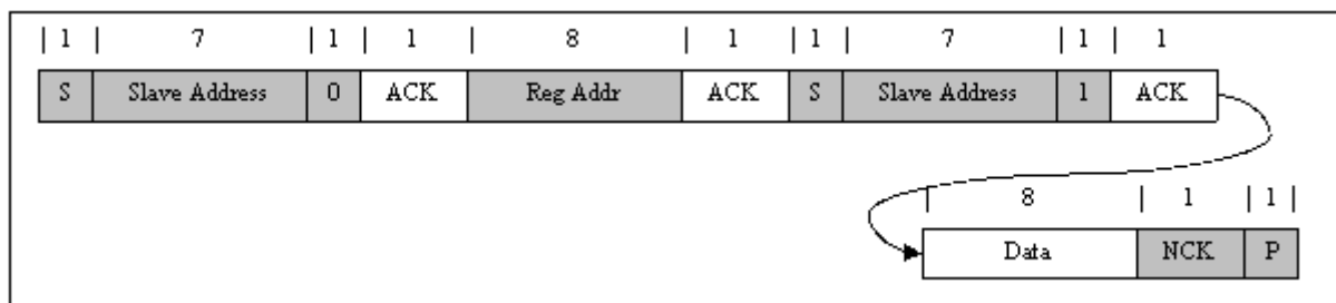
图 9-13. Single Read
