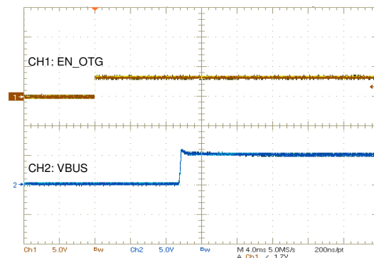
图 10-16. OTG Power Up from 8-V Battery
