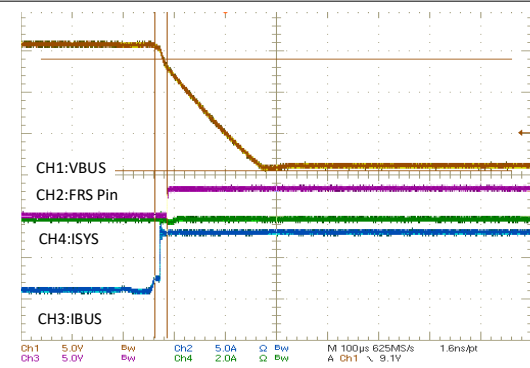
图 10-20. FRS Transition Waveform
