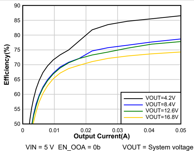
图 8-5. Light Load System Efficiency
