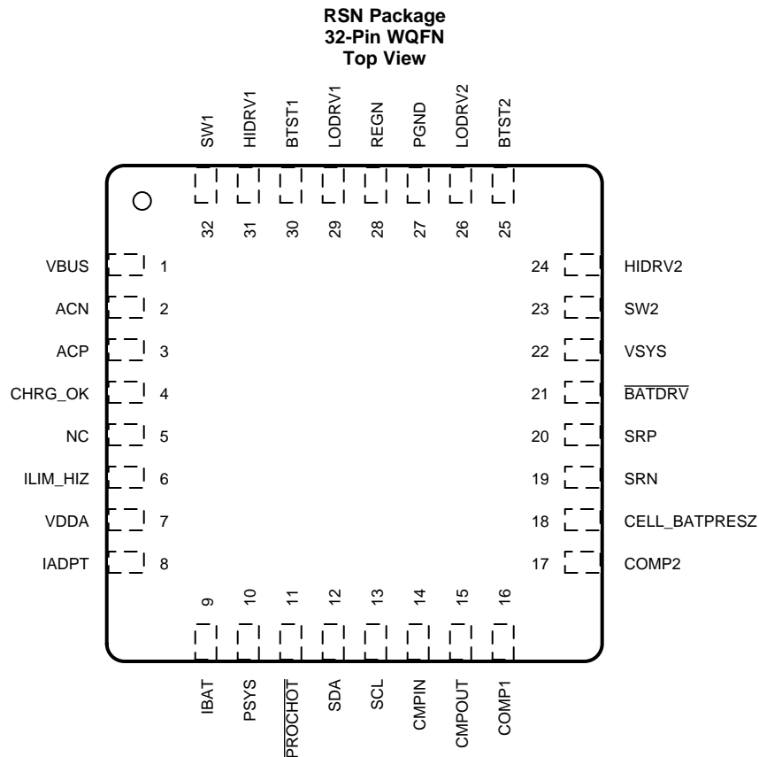
Pin Functions
