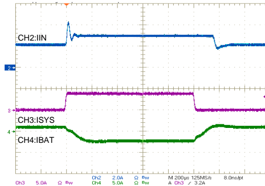
Figure 48. Input Current in Boost Mode
