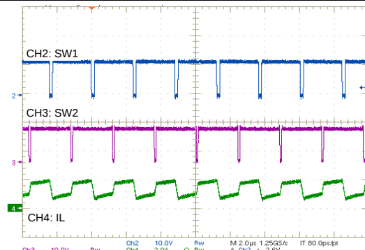
图 55. Switching During Buck Boost Mode
