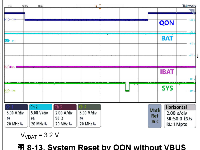
图 8-13. System Reset by QON without VBUS Present
