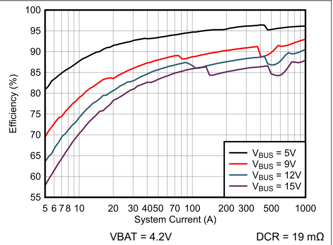
图 6-4. System Efficiency vs System Current
