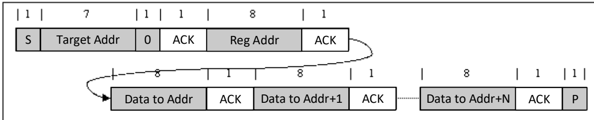
图 7-15. Multi-Write
