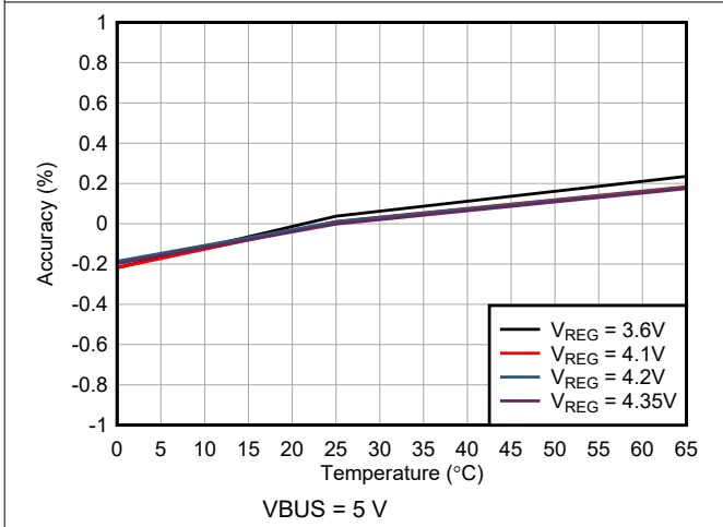
图 6-9. BAT Regulation Voltage vs Temperature
