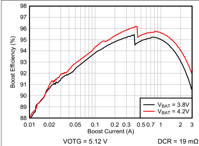
图 6-5. Boost Mode Efficiency vs VBUS Load Current
