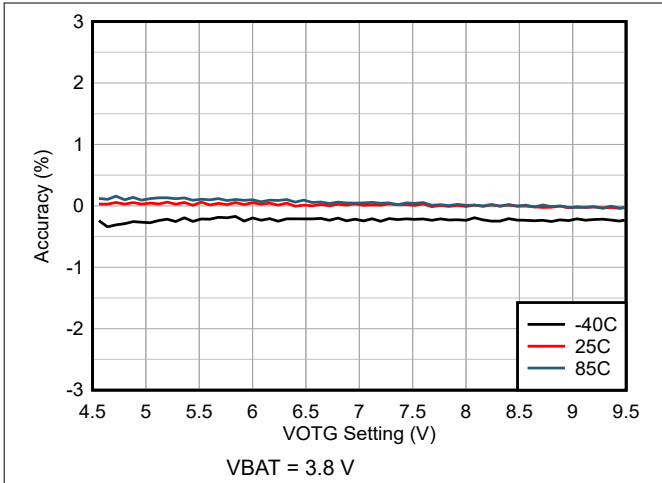
图 6-7. Boost Mode Voltage Accuracy vs VOTG I 2 C Setting
