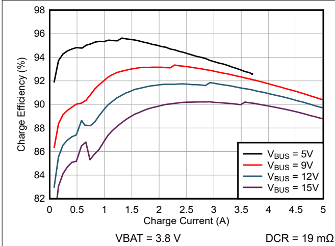
图 6-3. Charge Efficiency vs Charge Current
