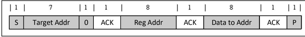
图 7-13. Single Write
