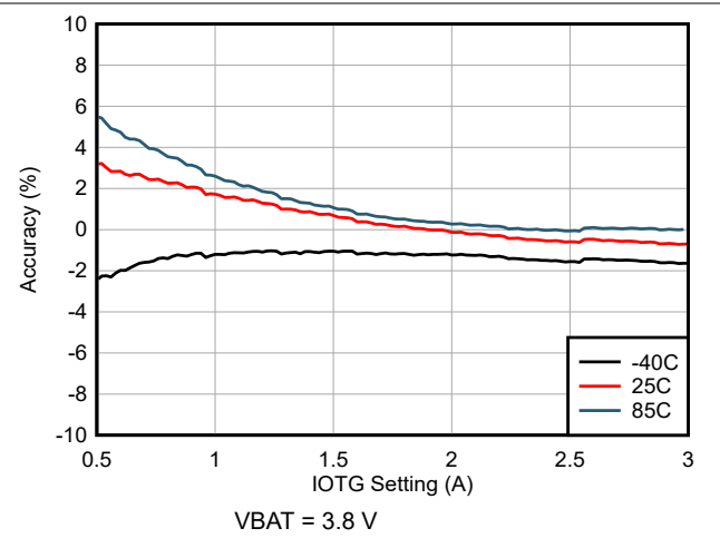
图 6-8. Boost Mode Current Limit Accuracy vs IOTG I 2 C Setting
