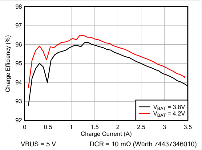
图 6-2. Charge Efficiency vs Charge Current
