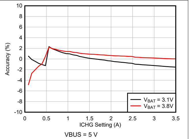
图 6-6. Charge Current Accuracy vs Charge Current I 2 C Setting
