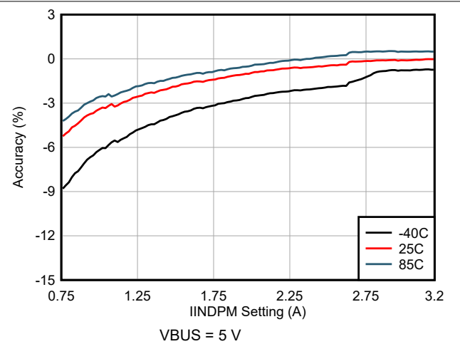
图 6-10. Input Current Limit vs IINDPM I 2 C Setting
