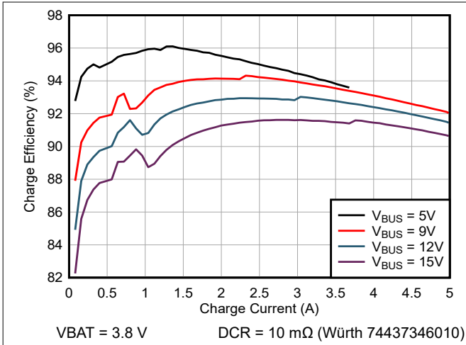
图 6-1. Charge Efficiency vs Charge Current
