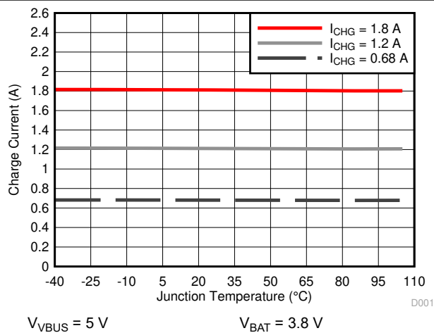
图 8-5. Charge Current vs. Junction Temperature
