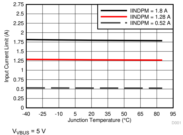
图 8-4. Input Current Limit vs. Junction Temperature
