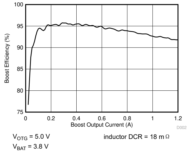
图 8-2. Efficiency vs. OTG Current
