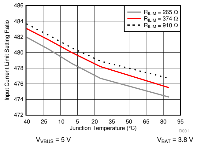
图 8-6. Input Current Limit Setting Ratio vs. Junction Temperature
