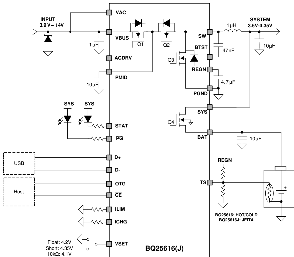
图 10-1. BQ25616/616J Application Diagram without External OVP
