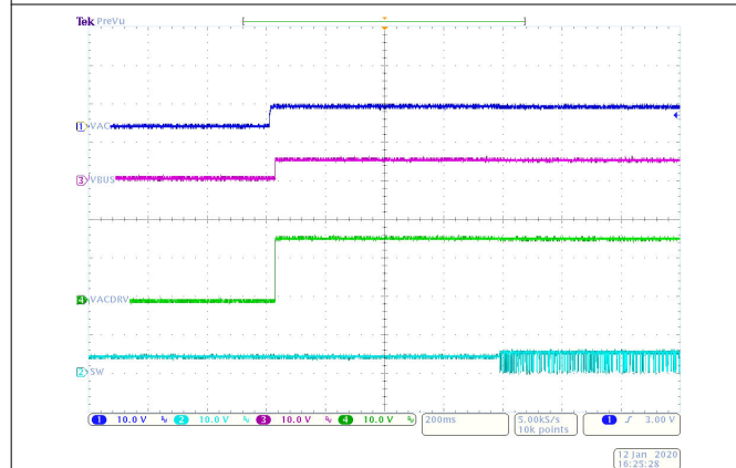
图 10-4. OVPFET Turn-on during Power-Up
