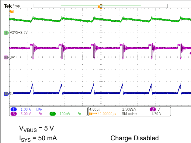
图 9-5. PFM Switching in Buck Mode
