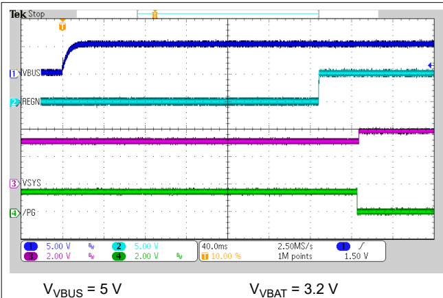
图 9-3. Power-Up with Charge Disabled
