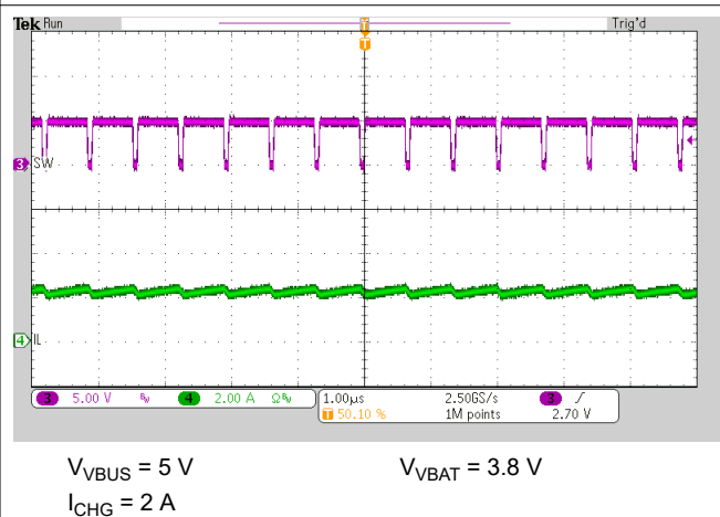
图 9-8. PWM Switching in Buck Mode
