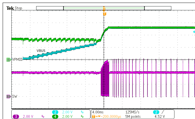
图 9-21. OTG Start-Up
