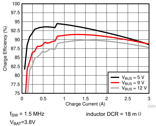
图 7-1. Charge Efficiency vs. Charge Current
