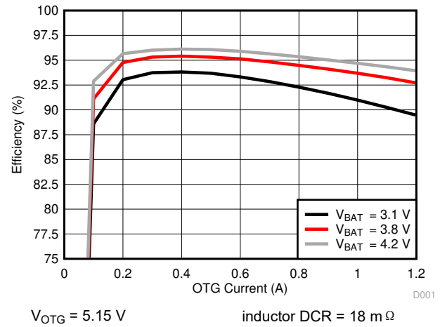
图 7-2. Efficiency vs. OTG Current
