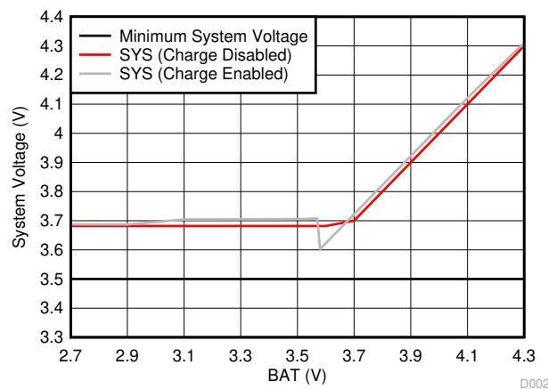
图 8-7. System Voltage vs Battery Voltage
