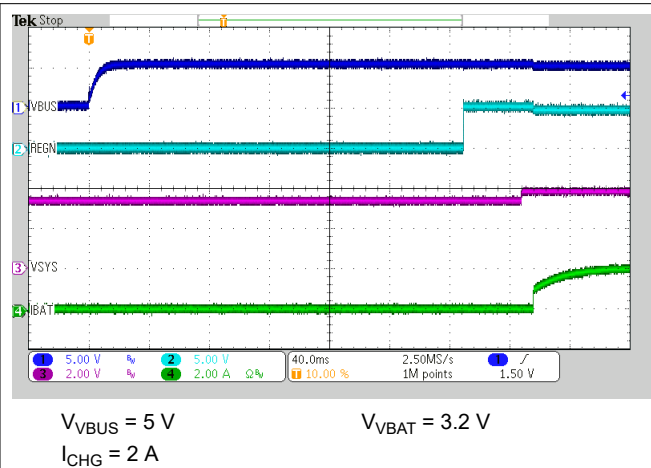
图 9-4. Power-Up with Charge Enabled
