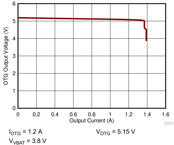
图 7-3. OTG Output Voltage vs. Output Current
