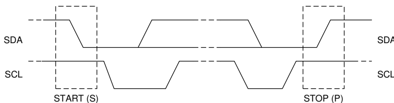
图 8-13. TS START and STOP conditions
