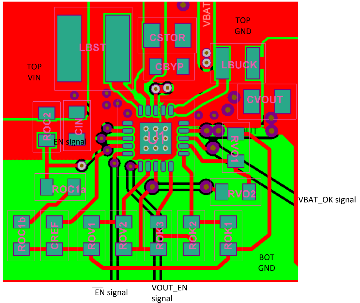
Figure 48. Layout Schematic
