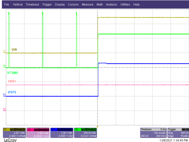
图 9-2. Power Up with IN Supply Insertion with No Battery
