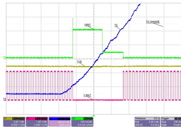
图 8-11. TS Change Response
