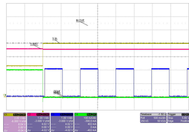
图 8-7. IN OVP Response
