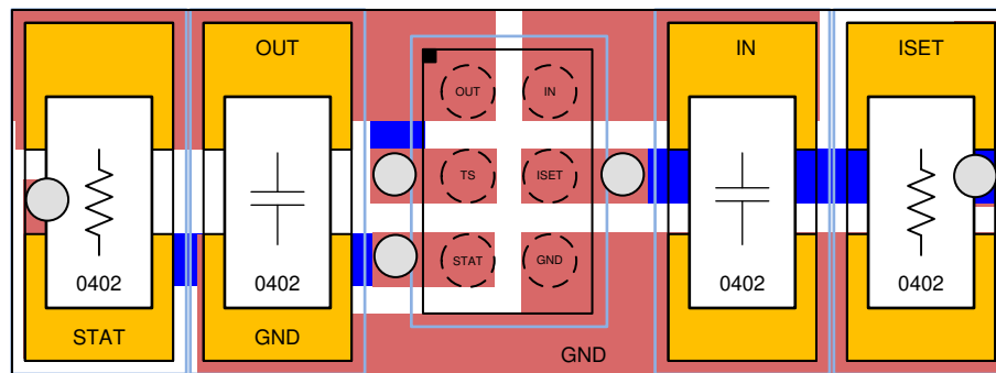
图 10-1. BQ25175 Board Layout Example
