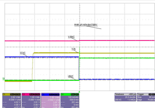
图 8-2. Power Up with Battery
