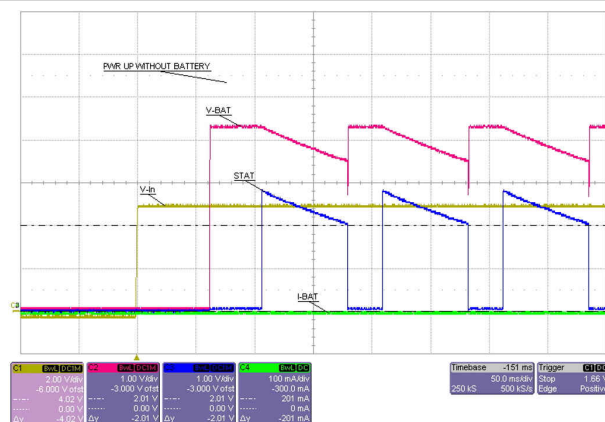
图 8-3. Power Up without Battery
