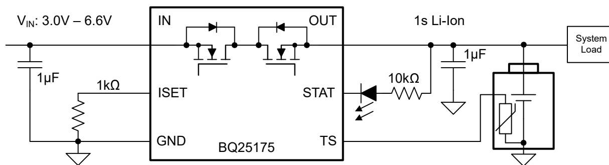
图 8-1. BQ25175 Typical Application for 1s Li-Ion Charging at 100 mA
