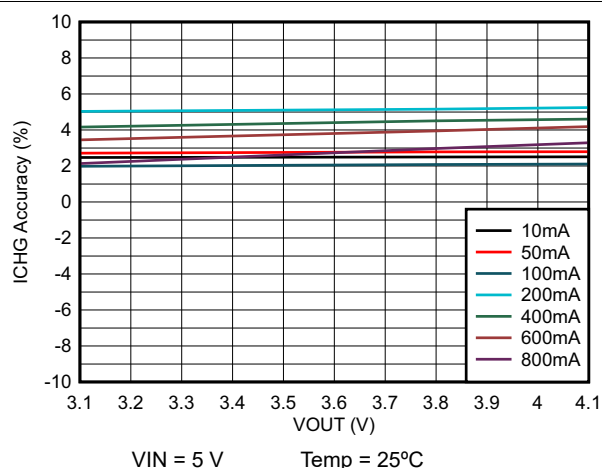
图 6-3. ICHG Accuracy vs. V_{OUT}
