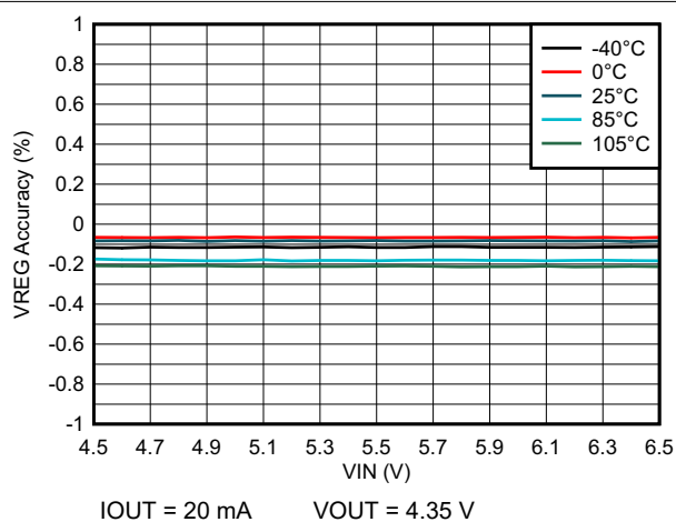
图 6-1. Line Regulation
