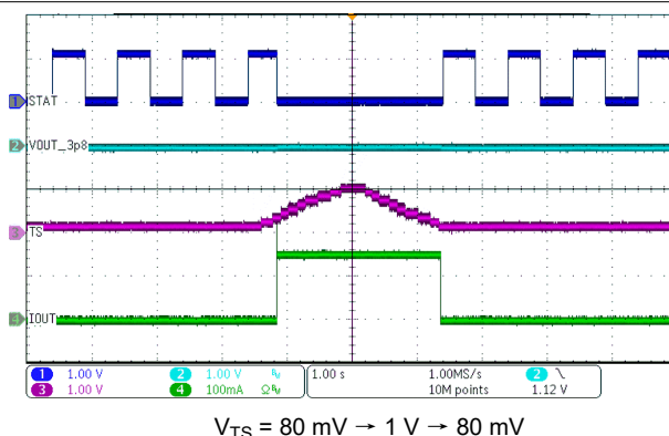
图 8-13. TS Change Response
