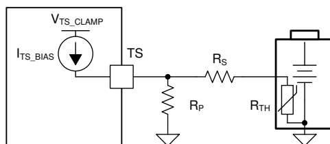
图 7-3. TS Resistor Network For Modified Temperature Charging Window
