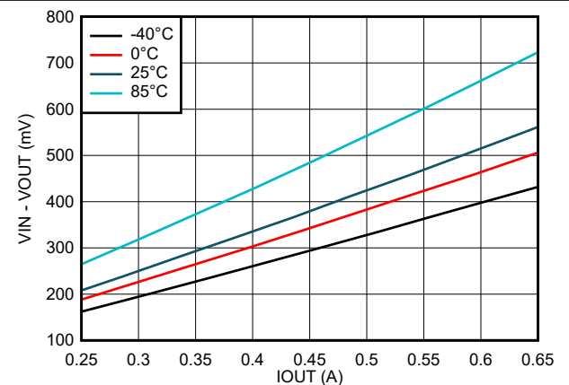
图 6-6. Dropout Voltage vs. Output Current
