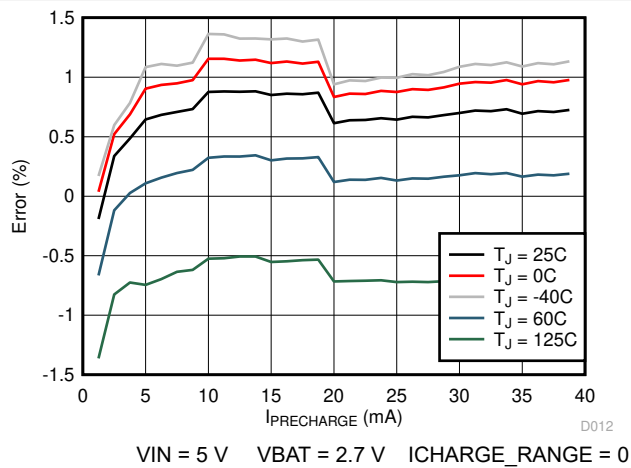
图 8-3. Pre-Charge Current Accuracy vs. IPRECHARGE setting (ICHARGE_RANGE = 0)
