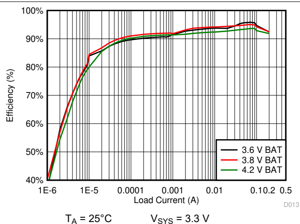
图 10-12. 3.3 V_{\text{SYS}} System Efficiency
