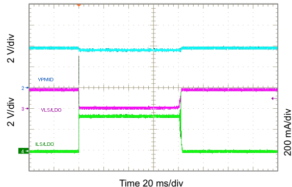
图 10-56. Short Circuit and Recovery for LDO
