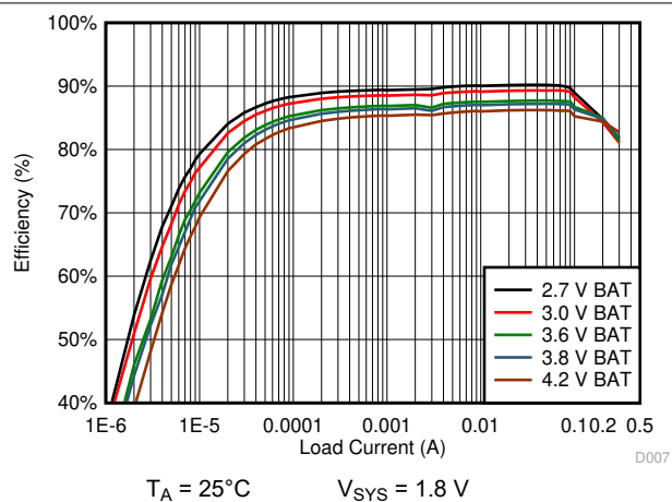
图 10-10. 1.8 V_{\text{SYS}} System Efficiency
