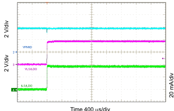
图 10-44. Startup Showing SS on LS/LDO Output
