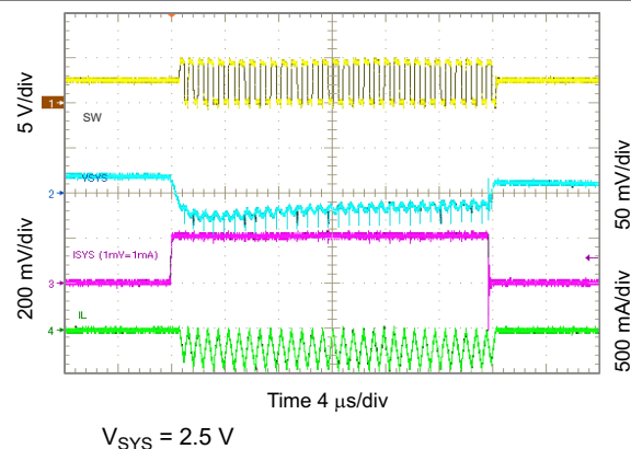
图 10-39. 2.5 V SYS Load Transient, 0 to 200 mA
