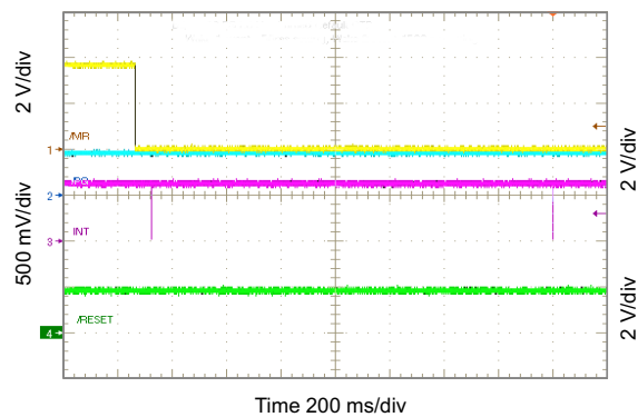
图 10-60. \overline{PG} Functions as Shifted \overline{MR} Output
