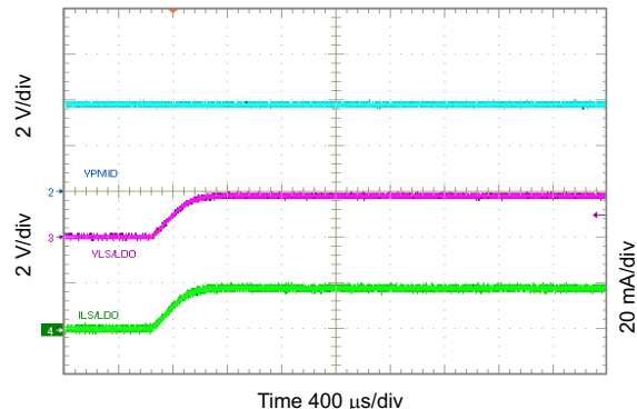
图 10-55. Startup Showing SS on LS/LDO in LDO Mode
