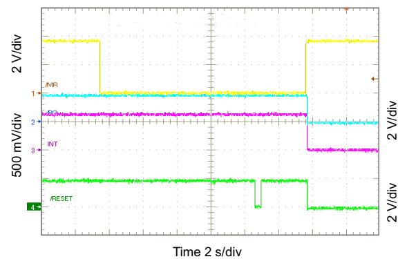
图 10-66. RESET Timing and Enter Ship Mode
