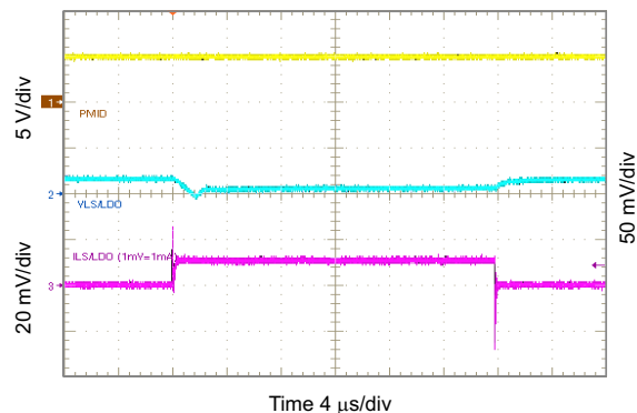
图 10-46. 1.2 V_{LSLDO} Load Transient, 0 to 10 mA
