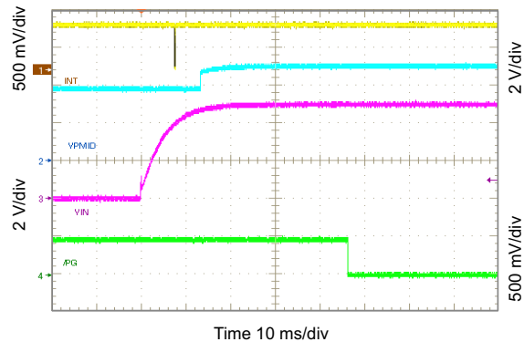
图 10-57. Show \overline{PG} and \overline{INT} Timing ( V_{IN} Insertion)
