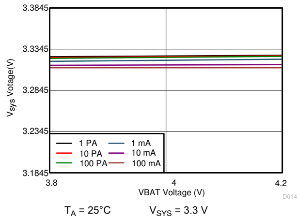
图 10-22. 3.3 V_{\text{SYS}} Line Regulation
