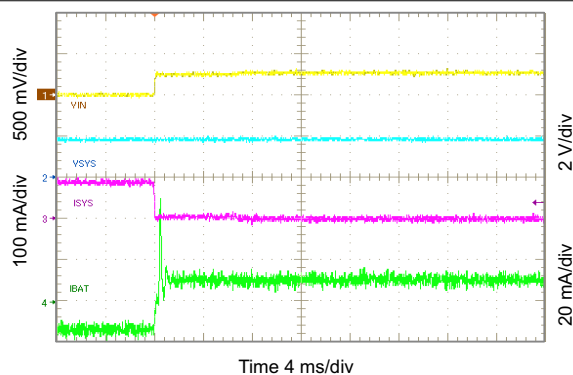
图 10-5. Exiting Battery Supplement Mode
