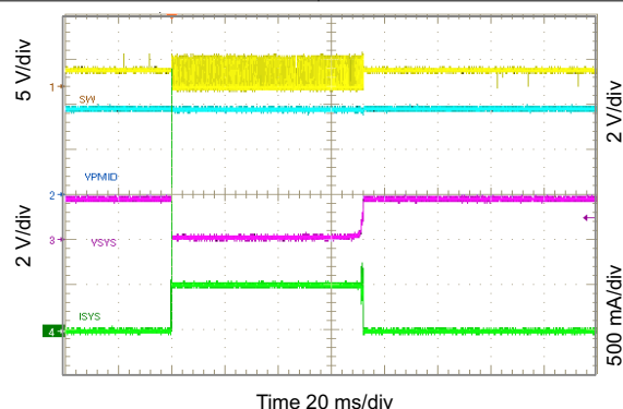
图 10-42. Short Circuit and Recovery for SYS
