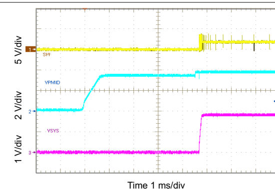
图 10-41. Startup Showing SS on SYS in PWM Mode
