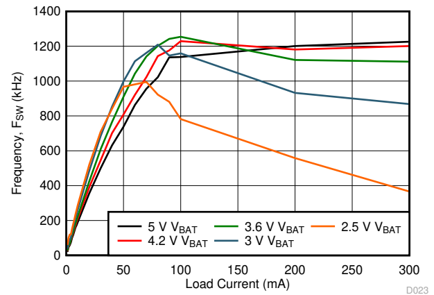
图 10-23. 1.8 V_{\text{SYS}} Switching Frequency vs Load Current
