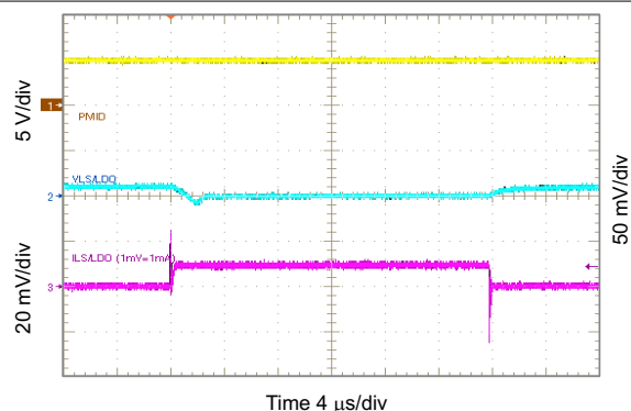
图 10-43. Short Circuit and Recovery for LS
