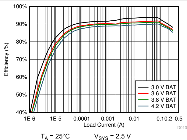
图 10-11. 2.5 V_{\text{SYS}} System Efficiency
