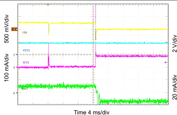
图 10-4. Entering Battery Supplement Mode
