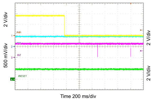
图 10-59. \overline{PG} Functions as Shifted \overline{MR} Output
